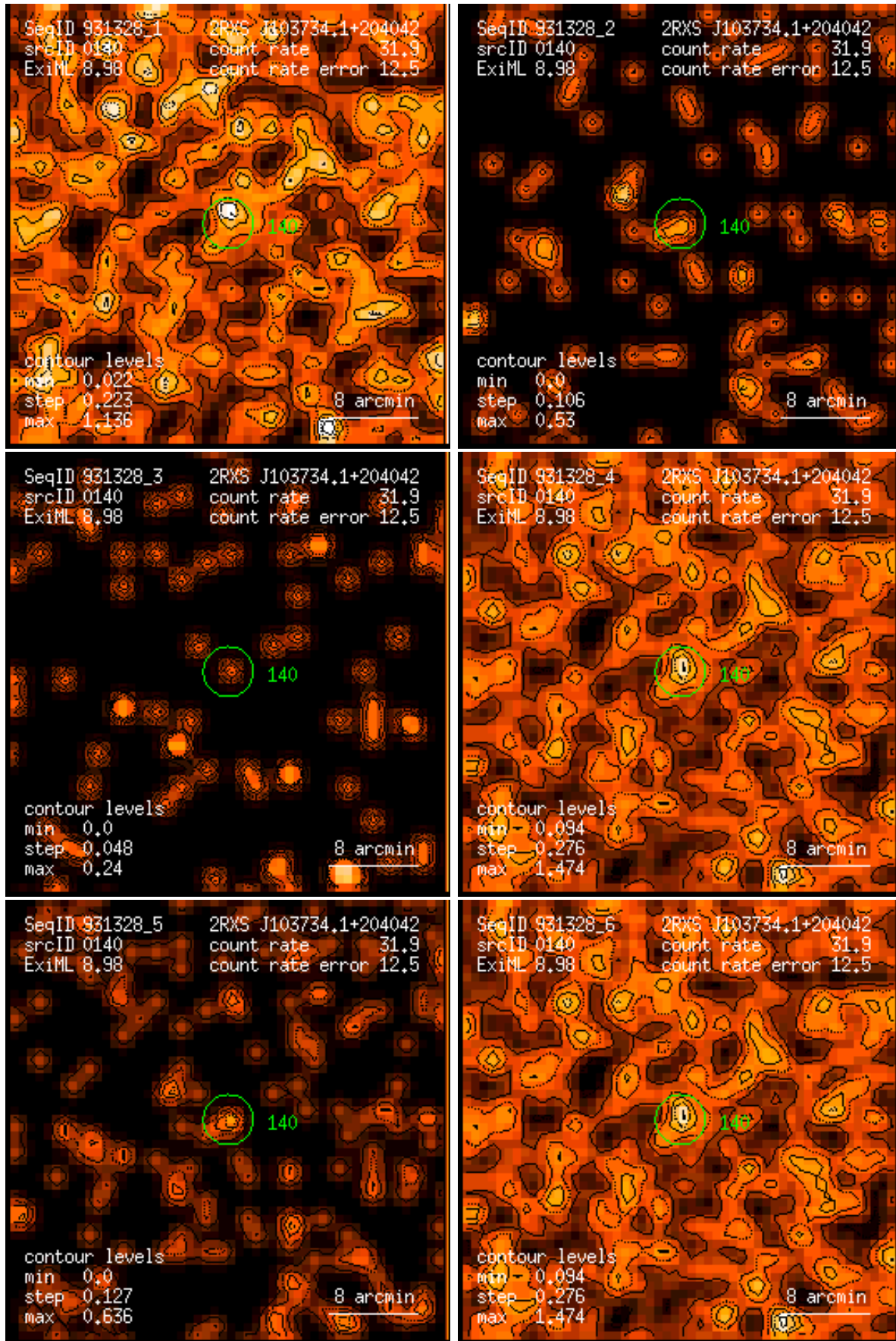
Figure 140: RASS 931328: detection 0140: band rate images, Gaussian filter: (1) PSPC channels 11 – 41, (2) 52 – 90, (3) 91 – 201, (4) 11 – 235, (5) 52 – 201, (6) 11 – 201. Broad band rates in counts/ks. Band rate contour levels in counts/ks/arcmin 2 .
