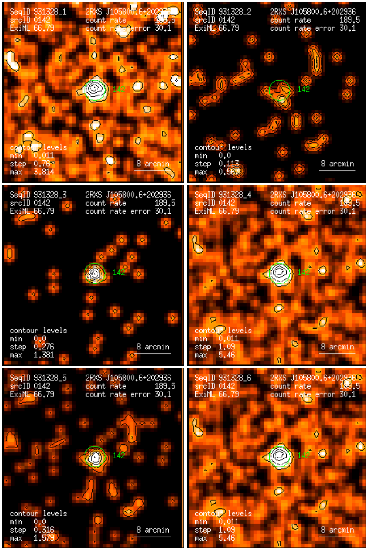
Figure 142: RASS 931328: detection 0142: band rate images, Gaussian filter: (1) PSPC channels 11 – 41, (2) 52 – 90, (3) 91 – 201, (4) 11 – 235, (5) 52 – 201, (6) 11 – 201. Broad band rates in counts/ks. Band rate contour levels in counts/ks/arcmin 2 .
