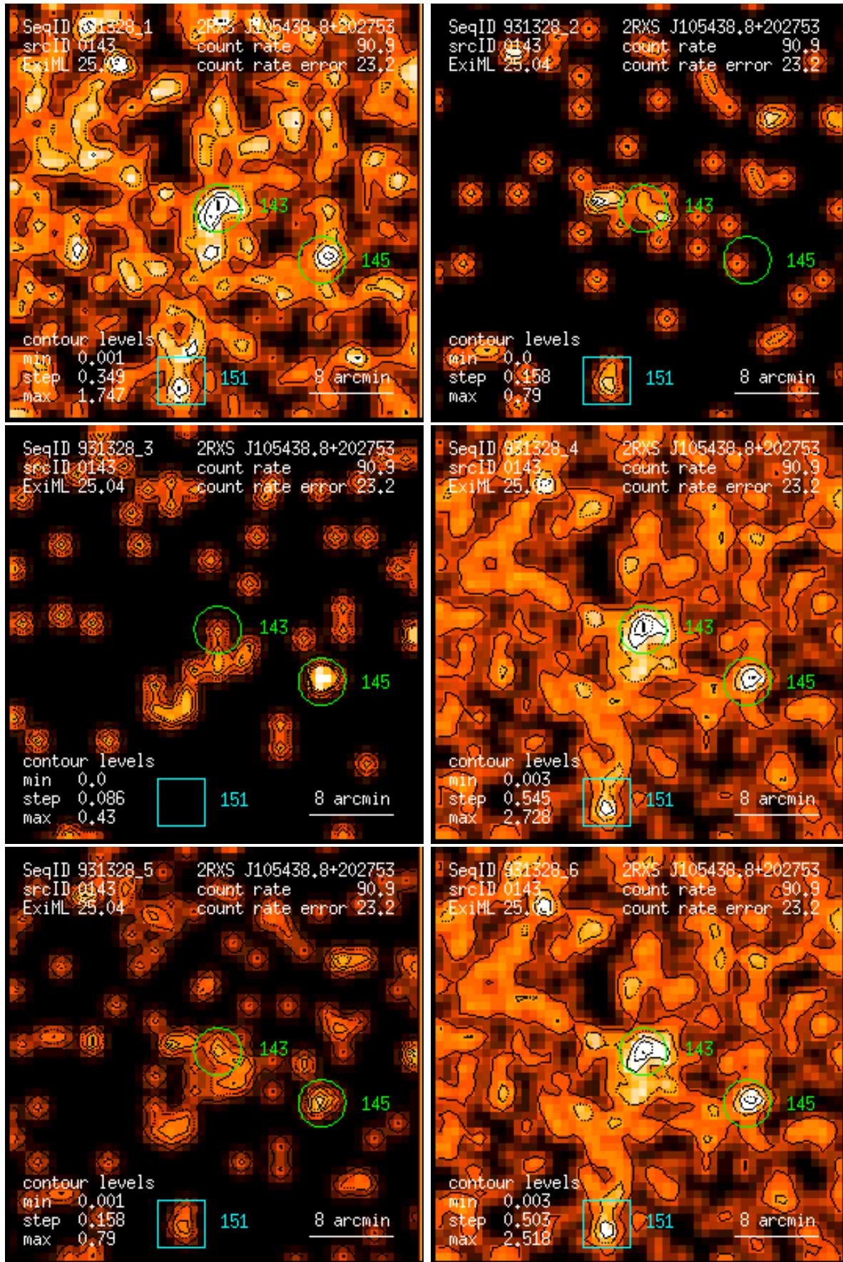
Figure 143: RASS 931328: detection 0143: band rate images, Gaussian filter: (1) PSPC channels 11 – 41, (2) 52 – 90, (3) 91 – 201, (4) 11 – 235, (5) 52 – 201, (6) 11 – 201. Broad band rates in counts/ks. Band rate contour levels in counts/ks/arcmin 2 .
