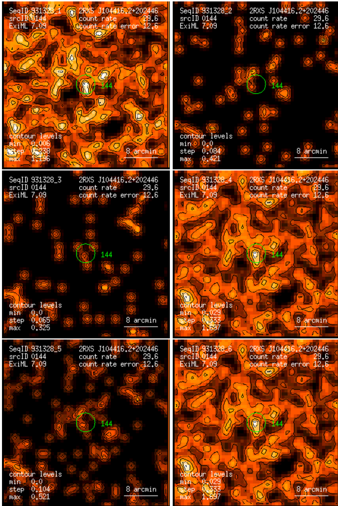
Figure 144: RASS 931328: detection 0144: band rate images, Gaussian filter: (1) PSPC channels 11 – 41, (2) 52 – 90, (3) 91 – 201, (4) 11 – 235, (5) 52 – 201, (6) 11 – 201. Broad band rates in counts/ks. Band rate contour levels in counts/ks/arcmin 2 .
