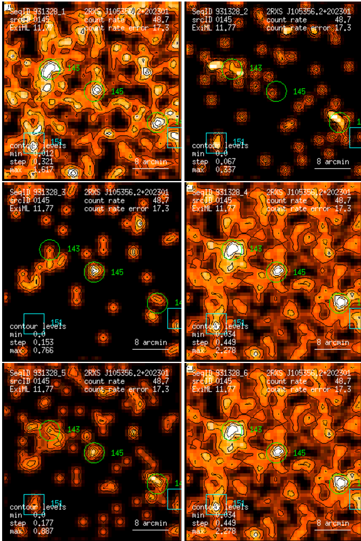
Figure 145: RASS 931328: detection 0145: band rate images, Gaussian filter: (1) PSPC channels 11 – 41, (2) 52 – 90, (3) 91 – 201, (4) 11 – 235, (5) 52 – 201, (6) 11 – 201. Broad band rates in counts/ks. Band rate contour levels in counts/ks/arcmin 2 .
