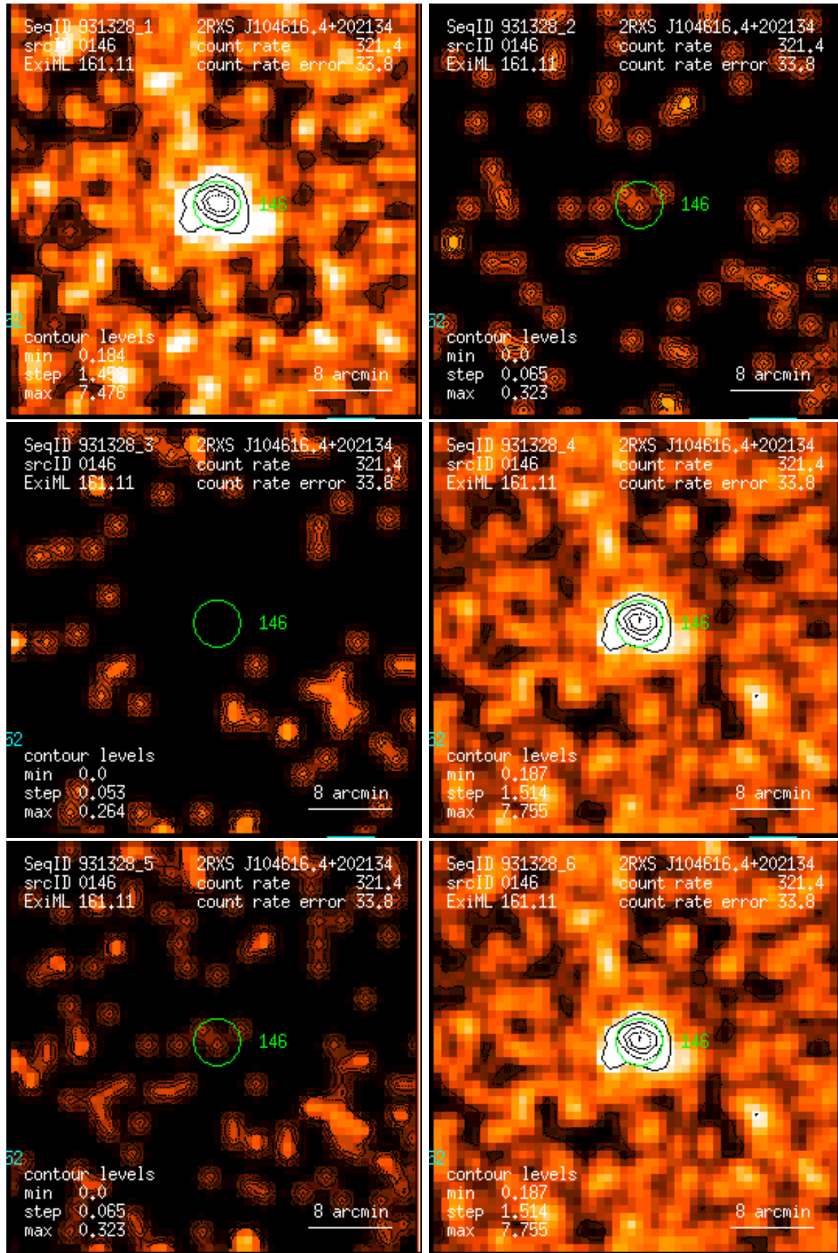
Figure 146: RASS 931328: detection 0146: band rate images, Gaussian filter: (1) PSPC channels 11 – 41, (2) 52 – 90, (3) 91 – 201, (4) 11 – 235, (5) 52 – 201, (6) 11 – 201. Broad band rates in counts/ks. Band rate contour levels in counts/ks/arcmin 2 .
