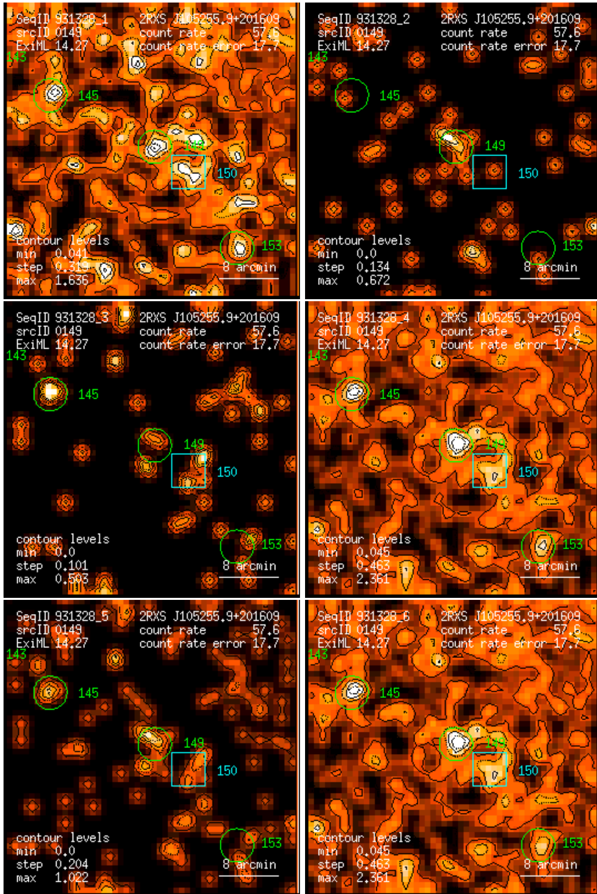
Figure 149: RASS 931328: detection 0149: band rate images, Gaussian filter: (1) PSPC channels 11 – 41, (2) 52 – 90, (3) 91 – 201, (4) 11 – 235, (5) 52 – 201, (6) 11 – 201. Broad band rates in counts/ks. Band rate contour levels in counts/ks/arcmin 2 .
