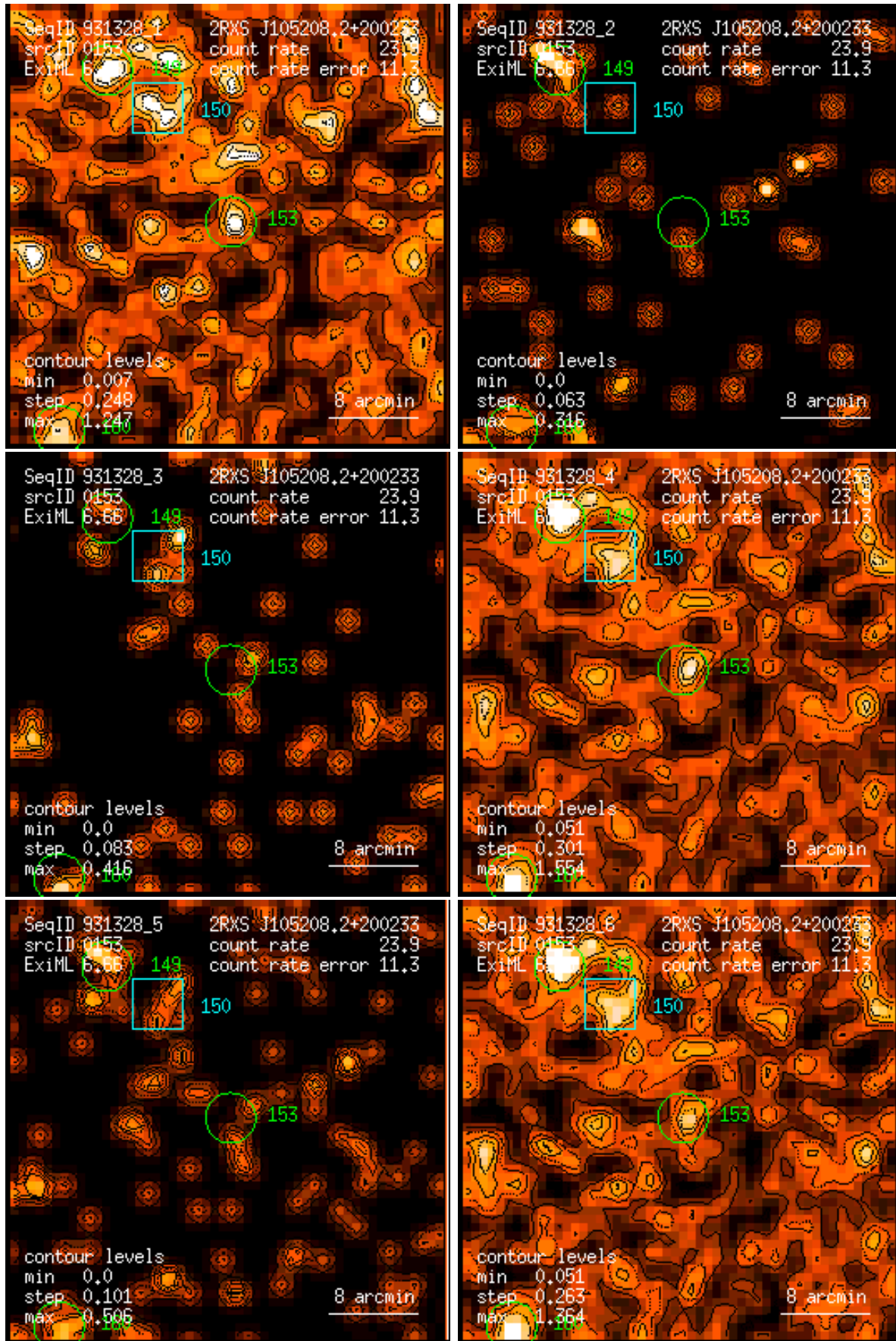
Figure 153: RASS 931328: detection 0153: band rate images, Gaussian filter: (1) PSPC channels 11 – 41, (2) 52 – 90, (3) 91 – 201, (4) 11 – 235, (5) 52 – 201, (6) 11 – 201. Broad band rates in counts/ks. Band rate contour levels in counts/ks/arcmin 2 .
