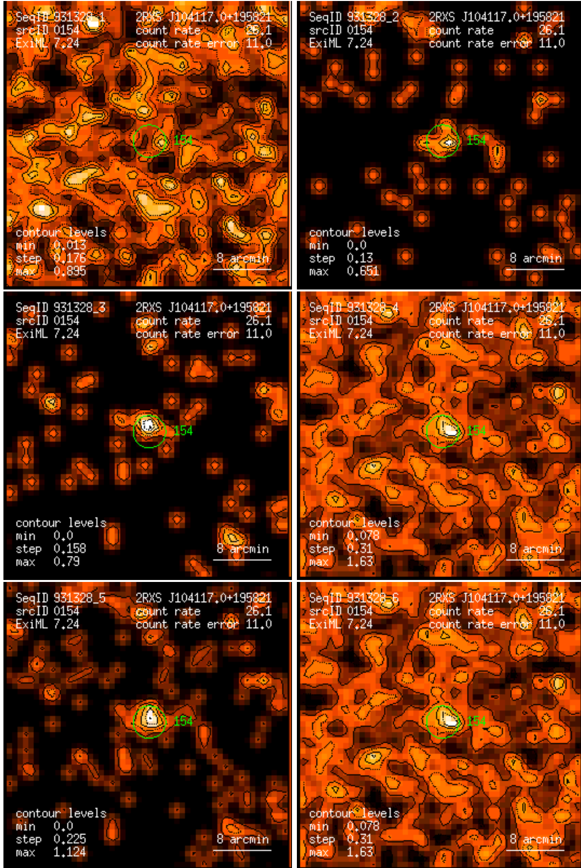
Figure 154: RASS 931328: detection 0154: band rate images, Gaussian filter: (1) PSPC channels 11 – 41, (2) 52 – 90, (3) 91 – 201, (4) 11 – 235, (5) 52 – 201, (6) 11 – 201. Broad band rates in counts/ks. Band rate contour levels in counts/ks/arcmin 2 .
