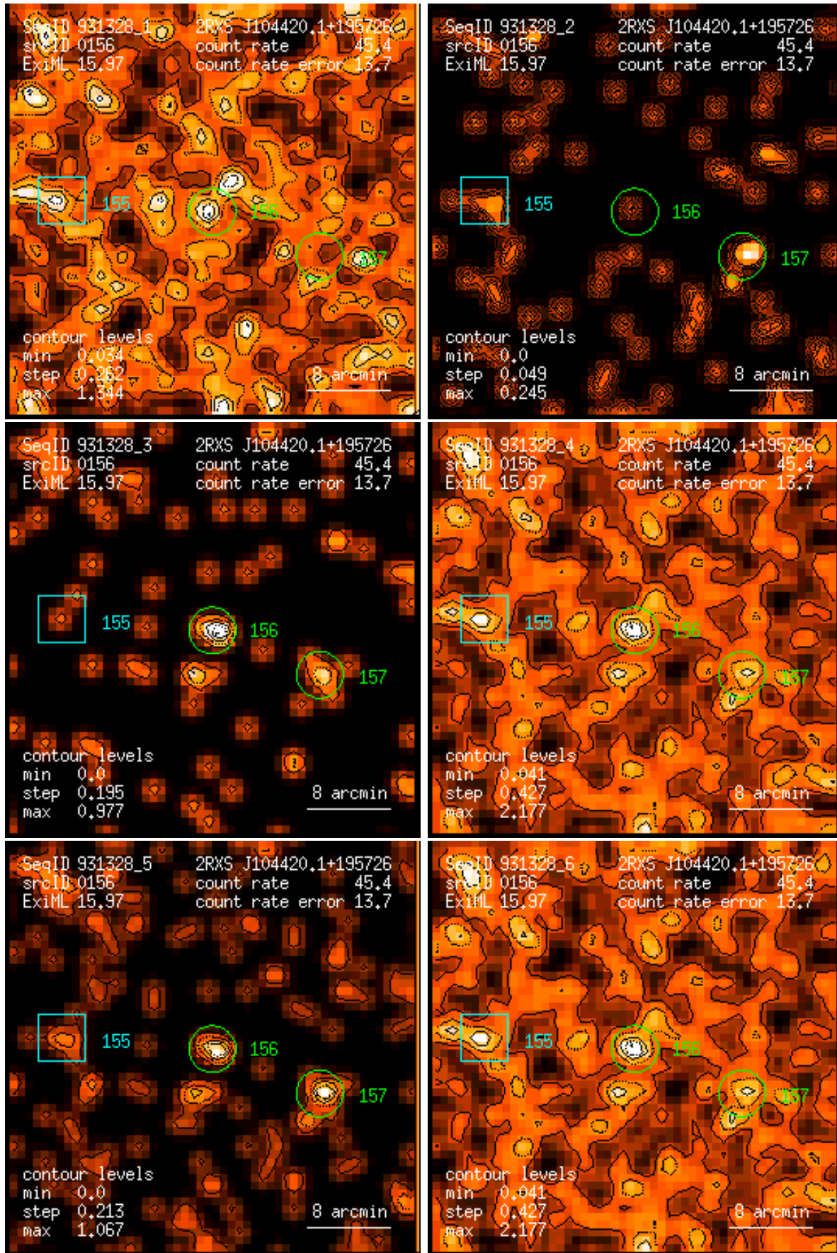
Figure 156: RASS 931328: detection 0156: band rate images, Gaussian filter: (1) PSPC channels 11 – 41, (2) 52 – 90, (3) 91 – 201, (4) 11 – 235, (5) 52 – 201, (6) 11 – 201. Broad band rates in counts/ks. Band rate contour levels in counts/ks/arcmin 2 .
