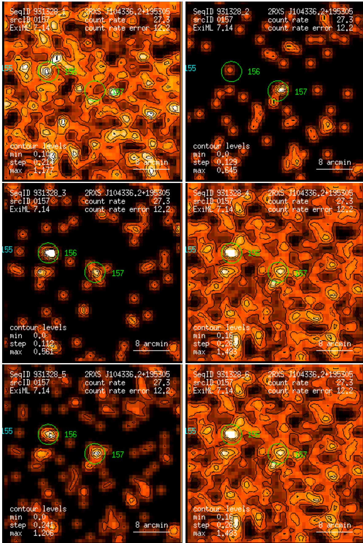
Figure 157: RASS 931328: detection 0157: band rate images, Gaussian filter: (1) PSPC channels 11 – 41, (2) 52 – 90, (3) 91 – 201, (4) 11 – 235, (5) 52 – 201, (6) 11 – 201. Broad band rates in counts/ks. Band rate contour levels in counts/ks/arcmin 2 .
