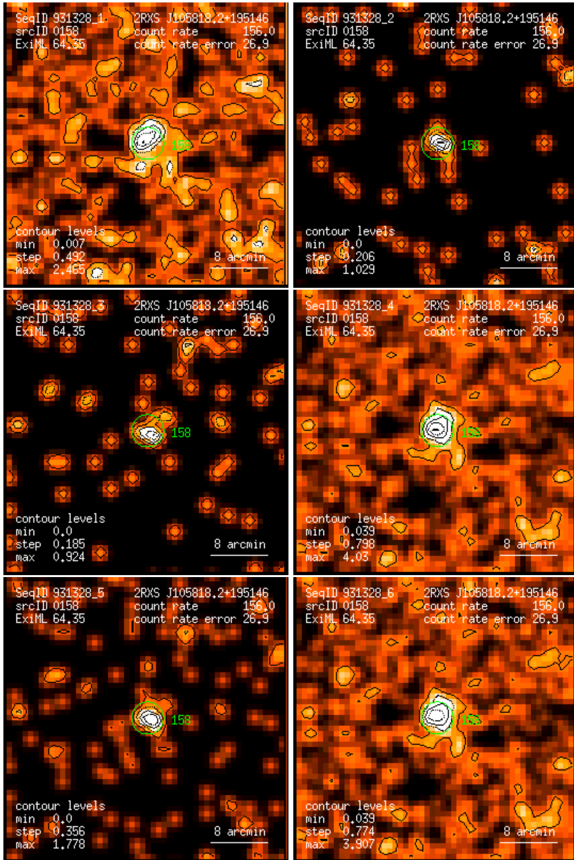
Figure 158: RASS 931328: detection 0158: band rate images, Gaussian filter: (1) PSPC channels 11 – 41, (2) 52 – 90, (3) 91 – 201, (4) 11 – 235, (5) 52 – 201, (6) 11 – 201. Broad band rates in counts/ks. Band rate contour levels in counts/ks/arcmin 2 .
