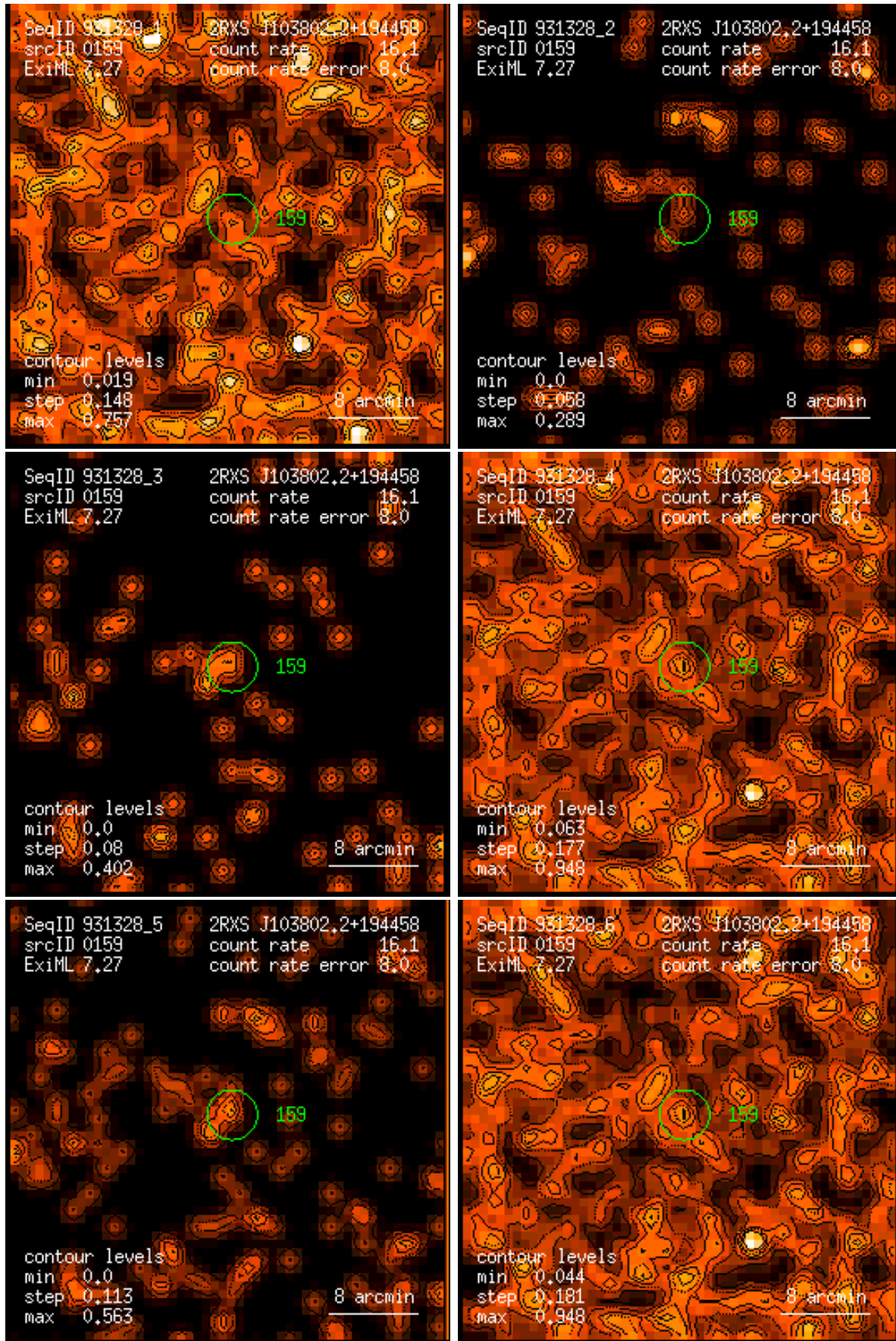
Figure 159: RASS 931328: detection 0159: band rate images, Gaussian filter: (1) PSPC channels 11 – 41, (2) 52 – 90, (3) 91 – 201, (4) 11 – 235, (5) 52 – 201, (6) 11 – 201. Broad band rates in counts/ks. Band rate contour levels in counts/ks/arcmin 2 .
