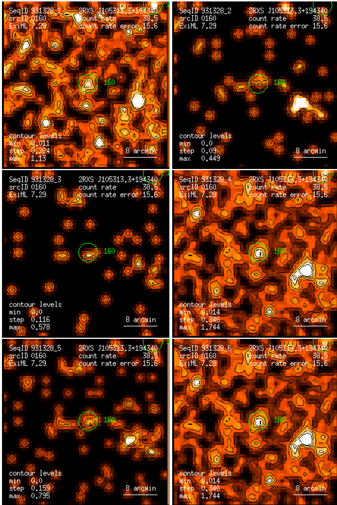
Figure 160: RASS 931328: detection 0160: band rate images, Gaussian filter: (1) PSPC channels 11 – 41, (2) 52 – 90, (3) 91 – 201, (4) 11 – 235, (5) 52 – 201, (6) 11 – 201. Broad band rates in counts/ks. Band rate contour levels in counts/ks/arcmin 2 .
