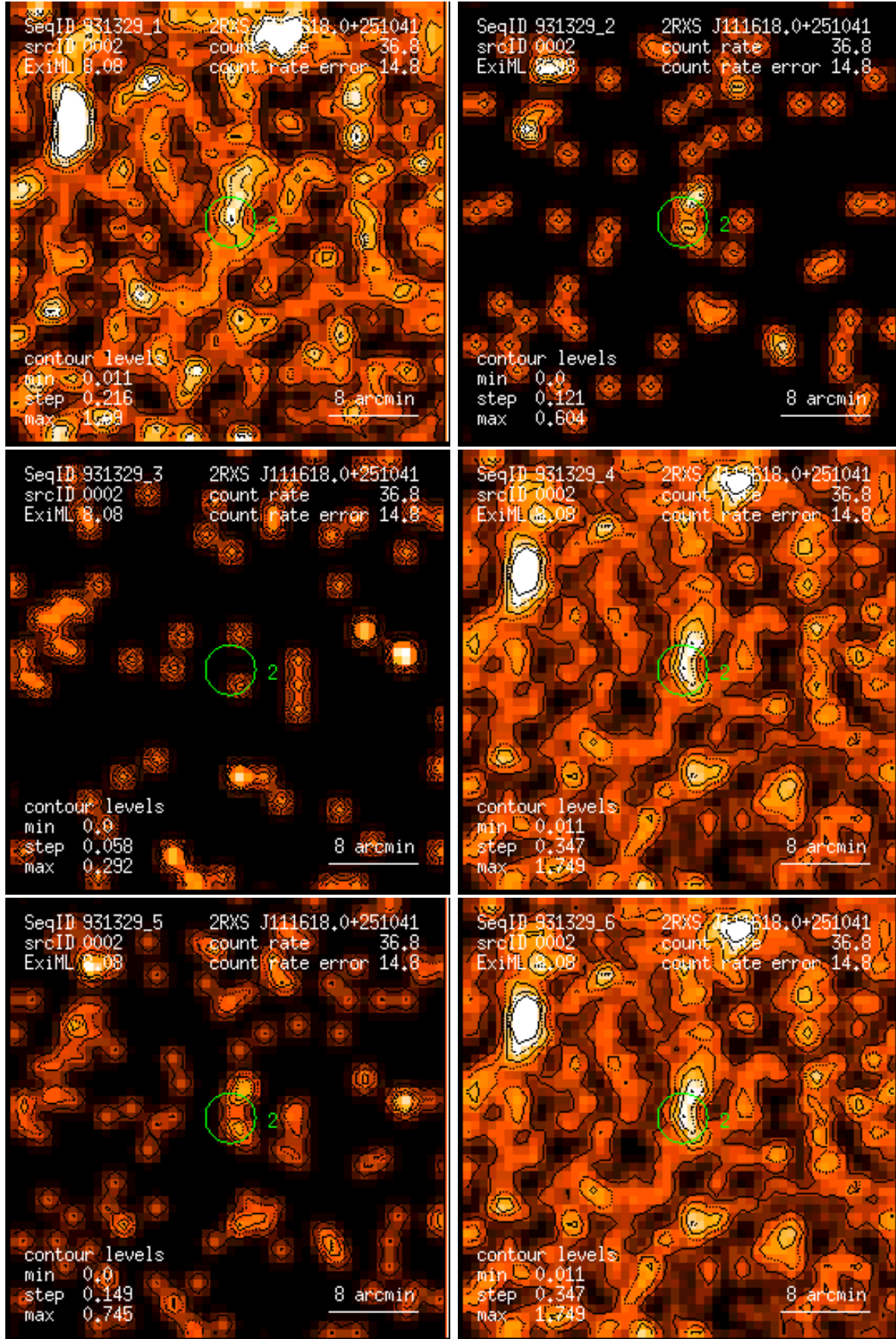
Figure 2: RASS 931329: detection 0002: band rate images, Gaussian filter: (1) PSPC channels 11 – 41, (2) 52 – 90, (3) 91 – 201, (4) 11 – 235, (5) 52 – 201, (6) 11 – 201. Broad band rates in counts/ks. Band rate contour levels in counts/ks/arcmin 2 .
