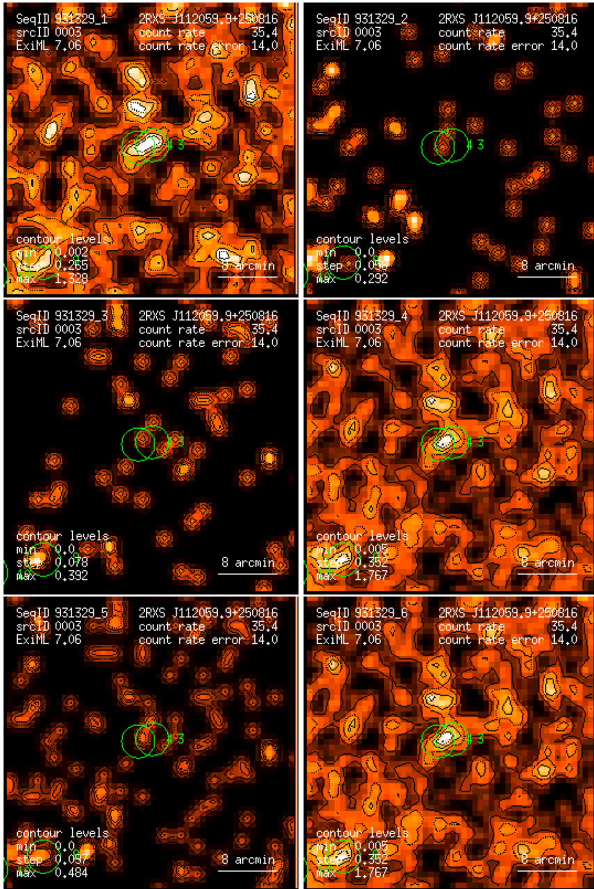
Figure 3: RASS 931329: detection 0003: band rate images, Gaussian filter: (1) PSPC channels 11 – 41, (2) 52 – 90, (3) 91 – 201, (4) 11 – 235, (5) 52 – 201, (6) 11 – 201. Broad band rates in counts/ks. Band rate contour levels in counts/ks/arcmin 2 .
