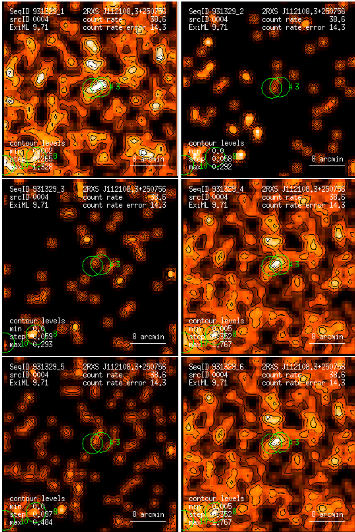
Figure 4: RASS 931329: detection 0004: band rate images, Gaussian filter: (1) PSPC channels 11 – 41, (2) 52 – 90, (3) 91 – 201, (4) 11 – 235, (5) 52 – 201, (6) 11 – 201. Broad band rates in counts/ks. Band rate contour levels in counts/ks/arcmin 2 .
