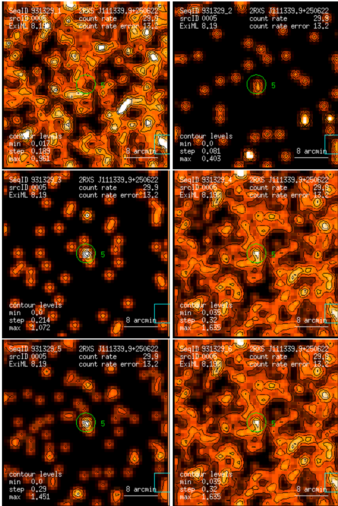
Figure 5: RASS 931329: detection 0005: band rate images, Gaussian filter: (1) PSPC channels 11 – 41, (2) 52 – 90, (3) 91 – 201, (4) 11 – 235, (5) 52 – 201, (6) 11 – 201. Broad band rates in counts/ks. Band rate contour levels in counts/ks/arcmin 2 .
