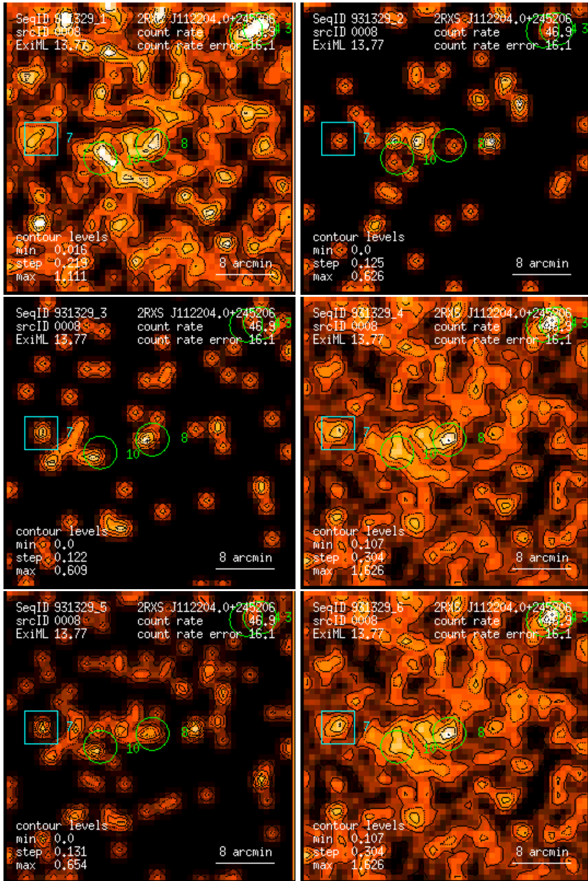
Figure 8: RASS 931329: detection 0008: band rate images, Gaussian filter: (1) PSPC channels 11 – 41, (2) 52 – 90, (3) 91 – 201, (4) 11 – 235, (5) 52 – 201, (6) 11 – 201. Broad band rates in counts/ks. Band rate contour levels in counts/ks/arcmin 2 .
