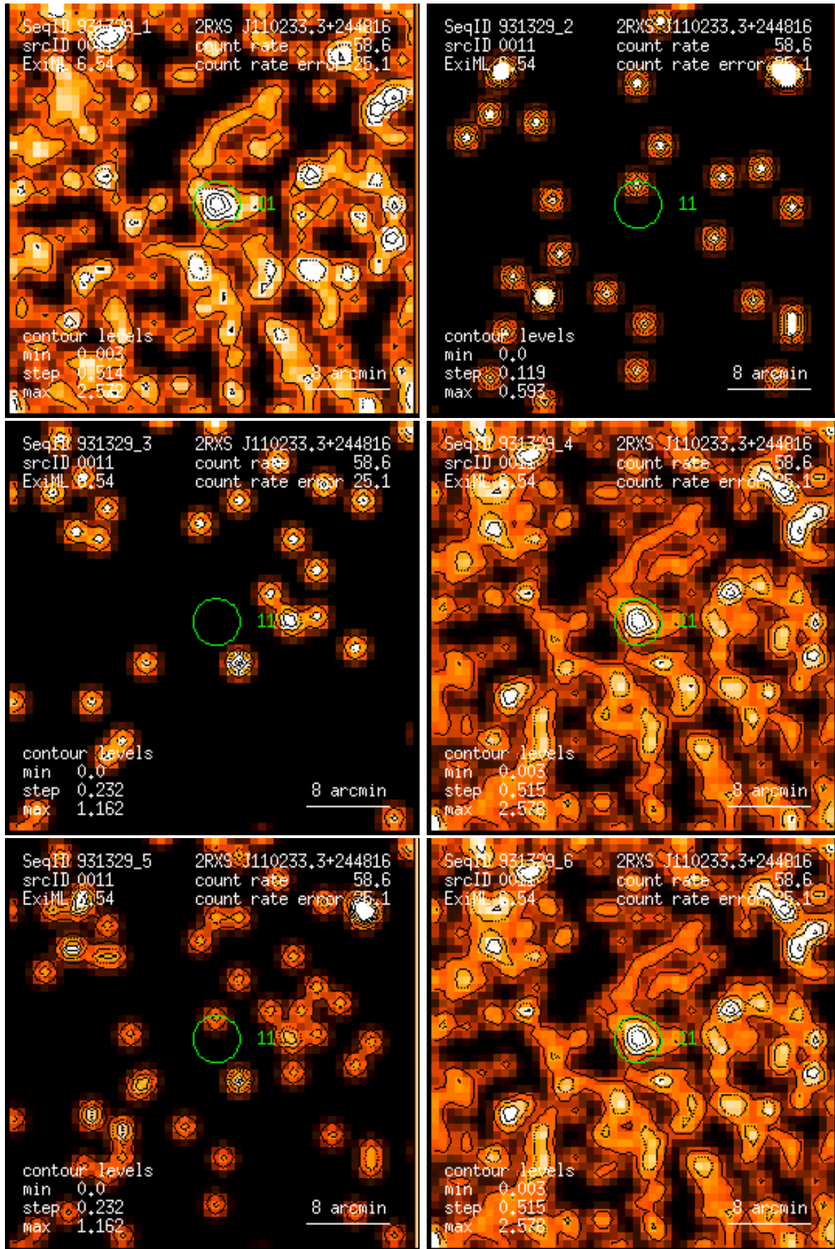
Figure 11: RASS 931329: detection 0011: band rate images, Gaussian filter: (1) PSPC channels 11 – 41, (2) 52 – 90, (3) 91 – 201, (4) 11 – 235, (5) 52 – 201, (6) 11 – 201. Broad band rates in counts/ks. Band rate contour levels in counts/ks/arcmin 2 .
