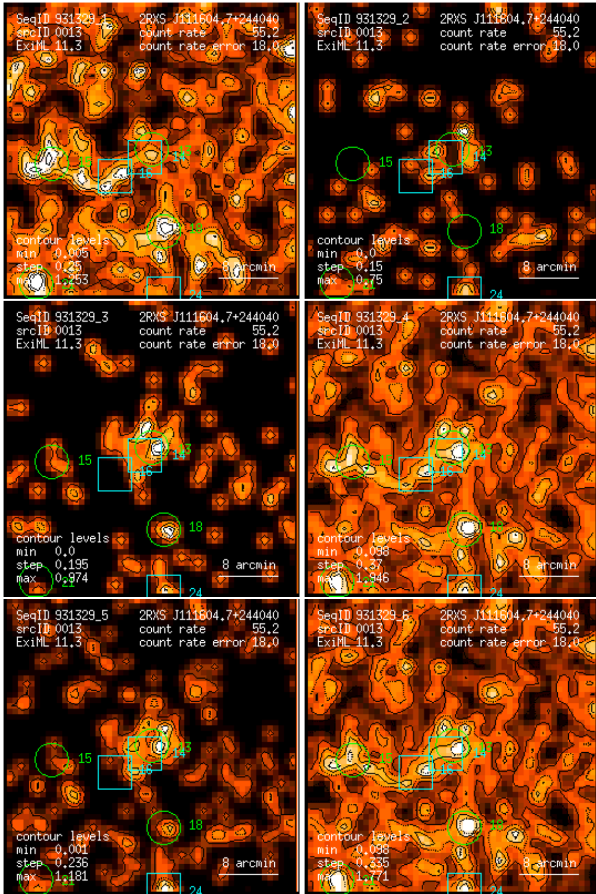
Figure 13: RASS 931329: detection 0013: band rate images, Gaussian filter: (1) PSPC channels 11 – 41, (2) 52 – 90, (3) 91 – 201, (4) 11 – 235, (5) 52 – 201, (6) 11 – 201. Broad band rates in counts/ks. Band rate contour levels in counts/ks/arcmin 2 .
