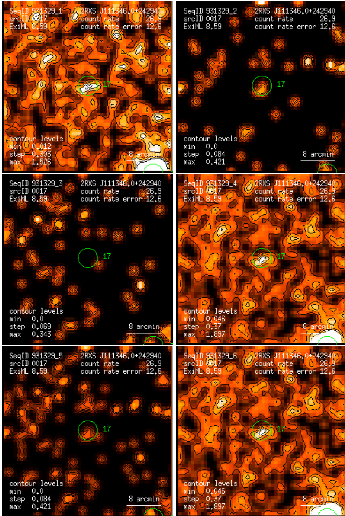
Figure 17: RASS 931329: detection 0017: band rate images, Gaussian filter: (1) PSPC channels 11 – 41, (2) 52 – 90, (3) 91 – 201, (4) 11 – 235, (5) 52 – 201, (6) 11 – 201. Broad band rates in counts/ks. Band rate contour levels in counts/ks/arcmin 2 .
