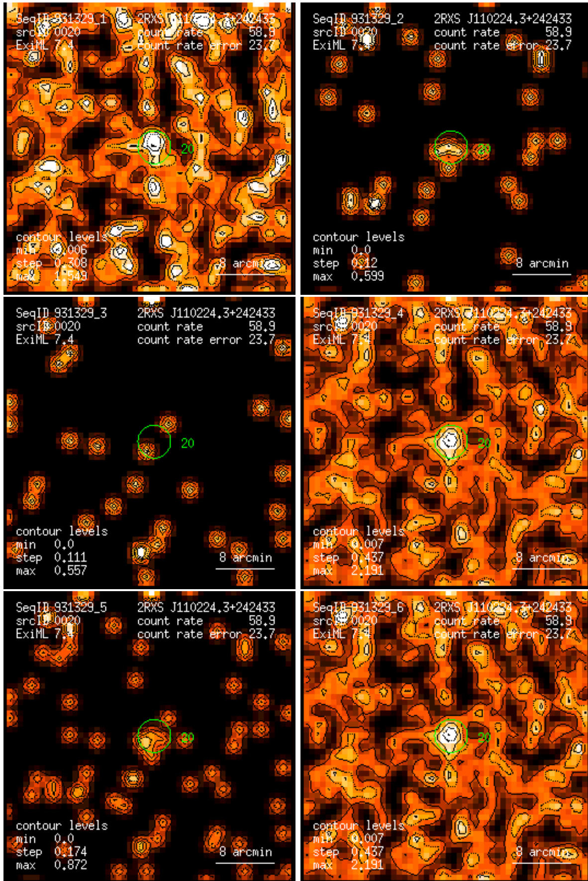
Figure 20: RASS 931329: detection 0020: band rate images, Gaussian filter: (1) PSPC channels 11 – 41, (2) 52 – 90, (3) 91 – 201, (4) 11 – 235, (5) 52 – 201, (6) 11 – 201. Broad band rates in counts/ks. Band rate contour levels in counts/ks/arcmin 2 .
