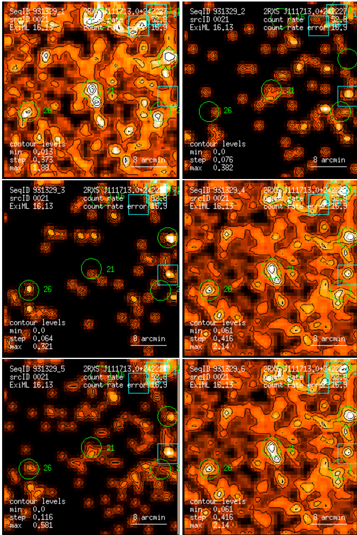
Figure 21: RASS 931329: detection 0021: band rate images, Gaussian filter: (1) PSPC channels 11 – 41, (2) 52 – 90, (3) 91 – 201, (4) 11 – 235, (5) 52 – 201, (6) 11 – 201. Broad band rates in counts/ks. Band rate contour levels in counts/ks/arcmin 2 .
