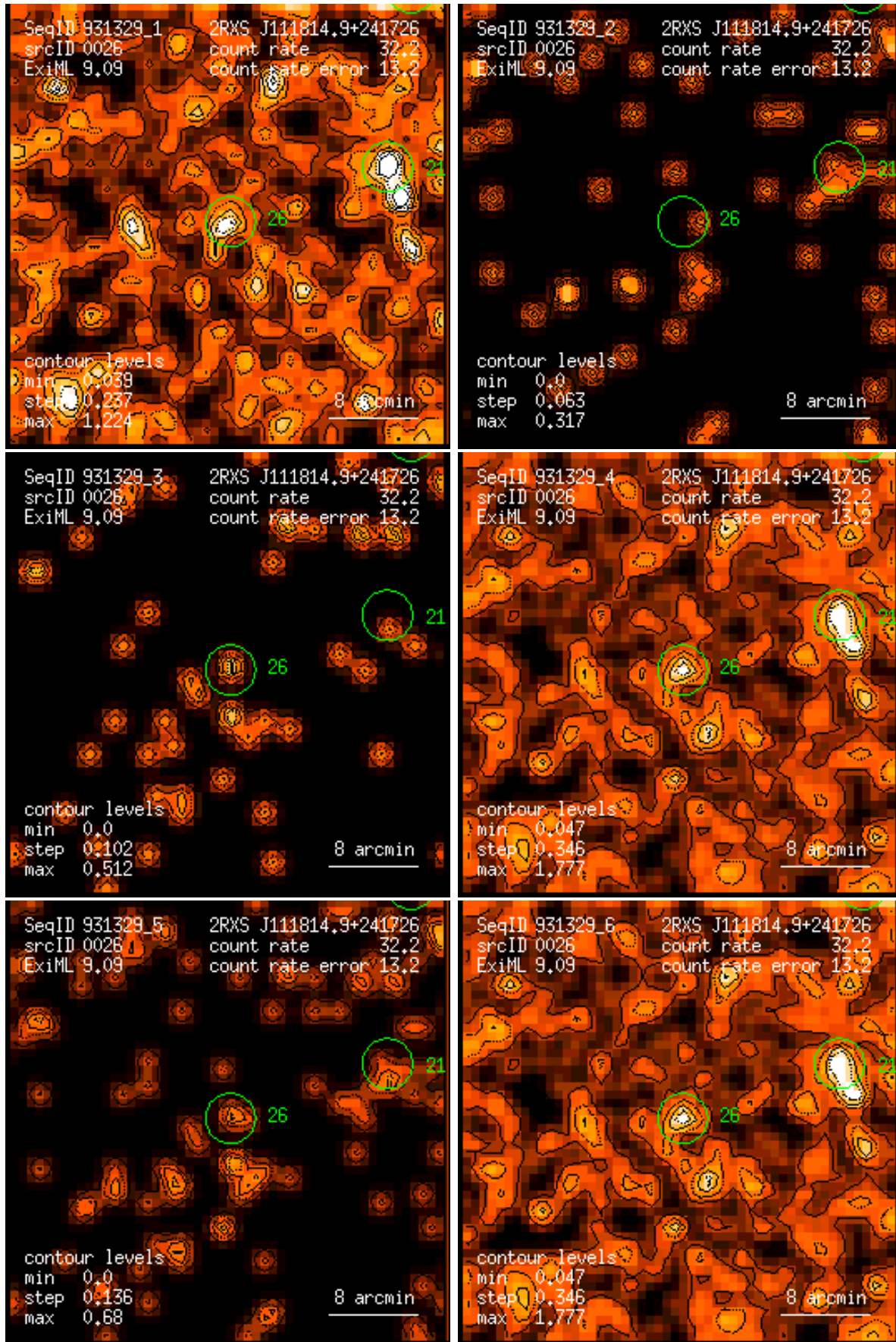
Figure 26: RASS 931329: detection 0026: band rate images, Gaussian filter: (1) PSPC channels 11 – 41, (2) 52 – 90, (3) 91 – 201, (4) 11 – 235, (5) 52 – 201, (6) 11 – 201. Broad band rates in counts/ks. Band rate contour levels in counts/ks/arcmin 2 .
