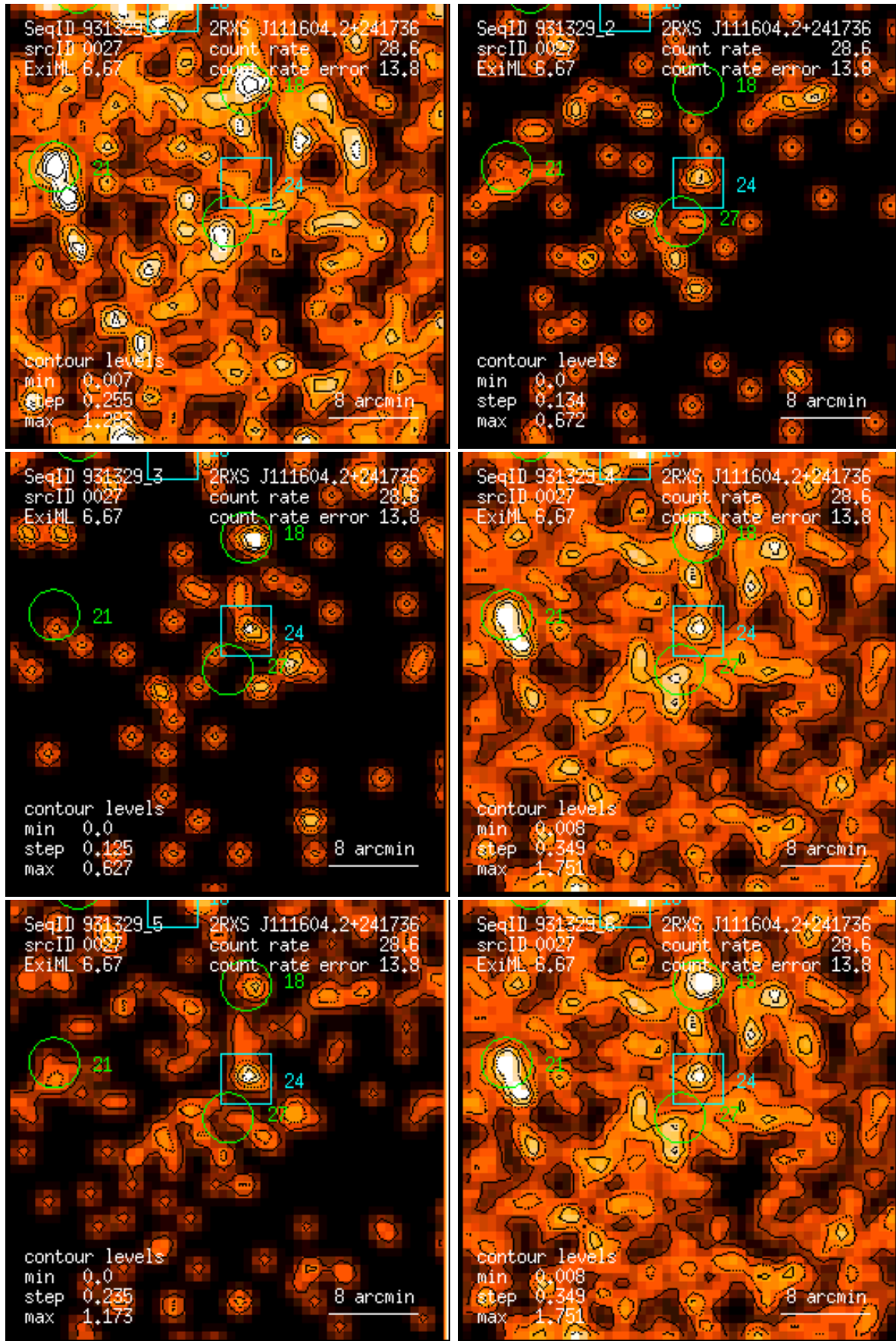
Figure 27: RASS 931329: detection 0027: band rate images, Gaussian filter: (1) PSPC channels 11 – 41, (2) 52 – 90, (3) 91 – 201, (4) 11 – 235, (5) 52 – 201, (6) 11 – 201. Broad band rates in counts/ks. Band rate contour levels in counts/ks/arcmin 2 .
