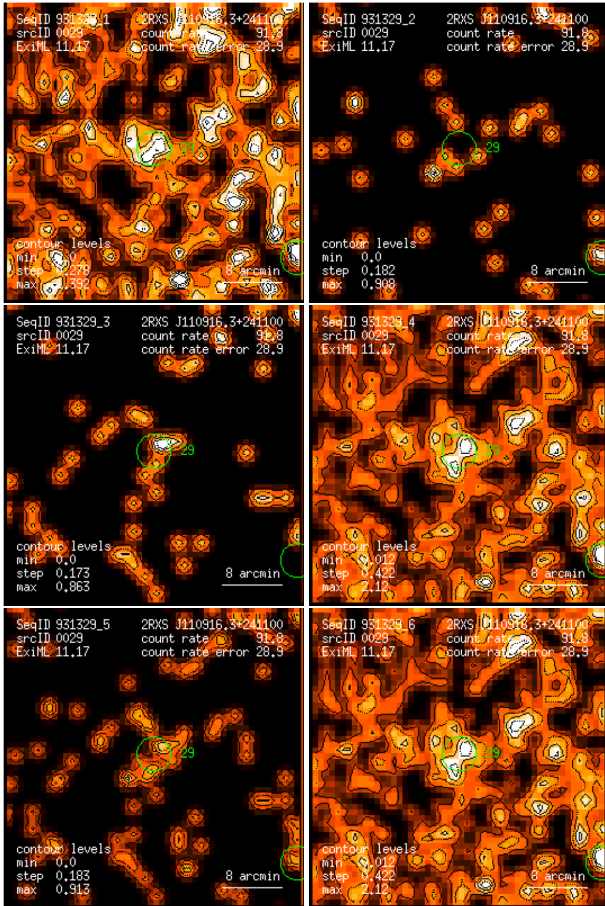
Figure 29: RASS 931329: detection 0029: band rate images, Gaussian filter: (1) PSPC channels 11 – 41, (2) 52 – 90, (3) 91 – 201, (4) 11 – 235, (5) 52 – 201, (6) 11 – 201. Broad band rates in counts/ks. Band rate contour levels in counts/ks/arcmin 2 .
