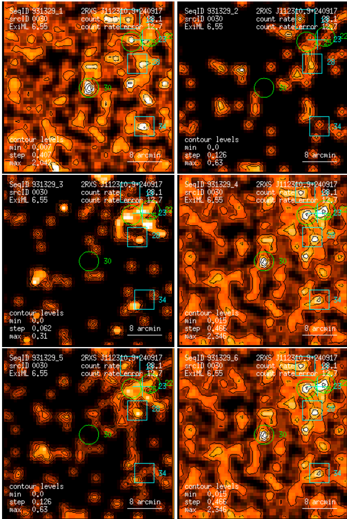
Figure 30: RASS 931329: detection 0030: band rate images, Gaussian filter: (1) PSPC channels 11 – 41, (2) 52 – 90, (3) 91 – 201, (4) 11 – 235, (5) 52 – 201, (6) 11 – 201. Broad band rates in counts/ks. Band rate contour levels in counts/ks/arcmin 2 .
