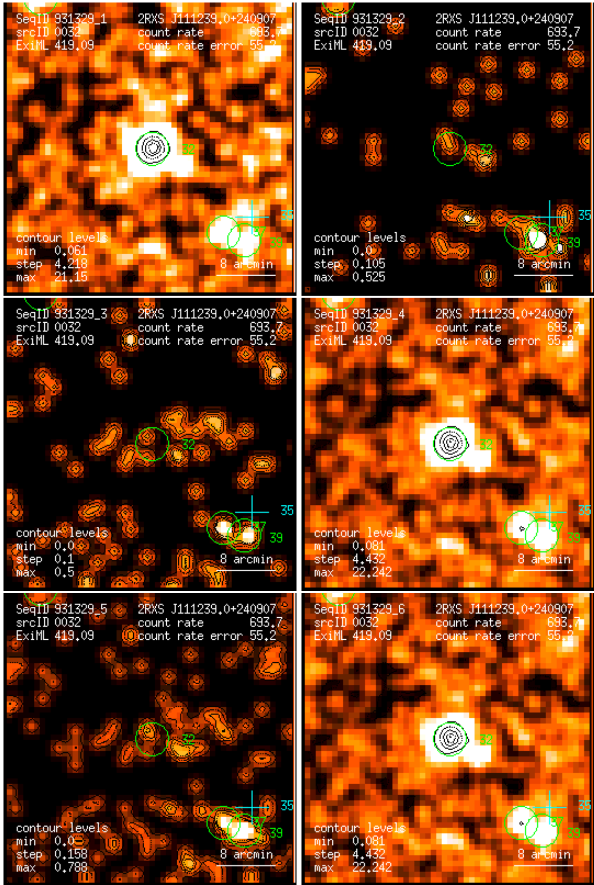
Figure 32: RASS 931329: detection 0032: band rate images, Gaussian filter: (1) PSPC channels 11 – 41, (2) 52 – 90, (3) 91 – 201, (4) 11 – 235, (5) 52 – 201, (6) 11 – 201. Broad band rates in counts/ks. Band rate contour levels in counts/ks/arcmin 2 .
