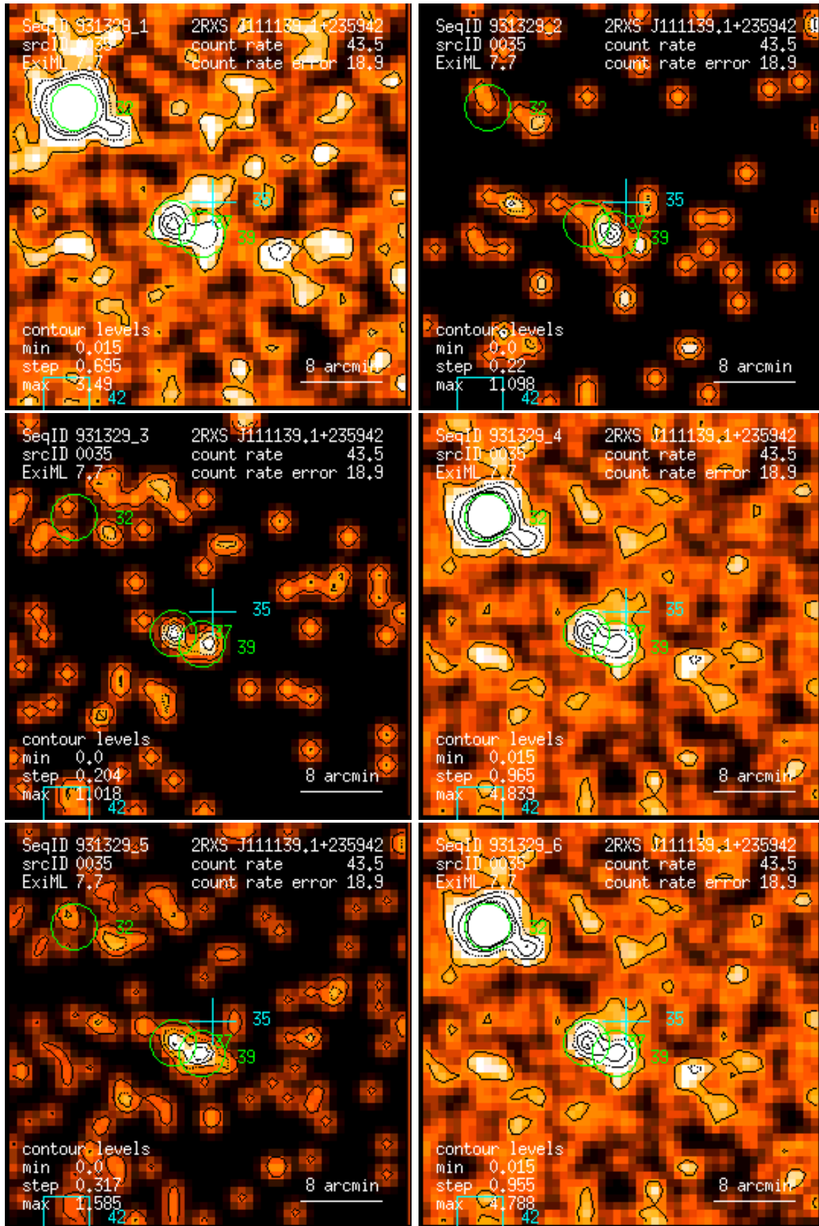
Figure 35: RASS 931329: detection 0035: band rate images, Gaussian filter: (1) PSPC channels 11 – 41, (2) 52 – 90, (3) 91 – 201, (4) 11 – 235, (5) 52 – 201, (6) 11 – 201. Broad band rates in counts/ks. Band rate contour levels in counts/ks/arcmin 2 .
