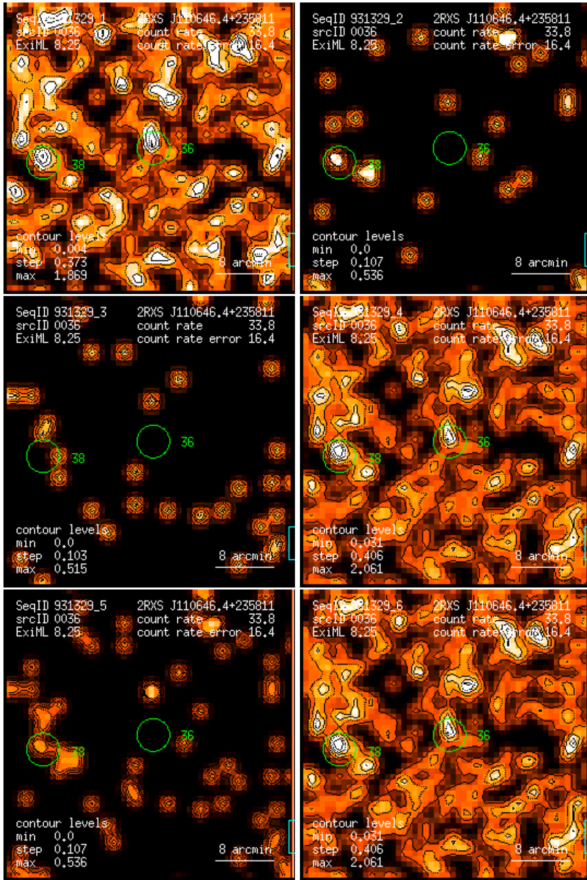
Figure 36: RASS 931329: detection 0036: band rate images, Gaussian filter: (1) PSPC channels 11 – 41, (2) 52 – 90, (3) 91 – 201, (4) 11 – 235, (5) 52 – 201, (6) 11 – 201. Broad band rates in counts/ks. Band rate contour levels in counts/ks/arcmin 2 .
