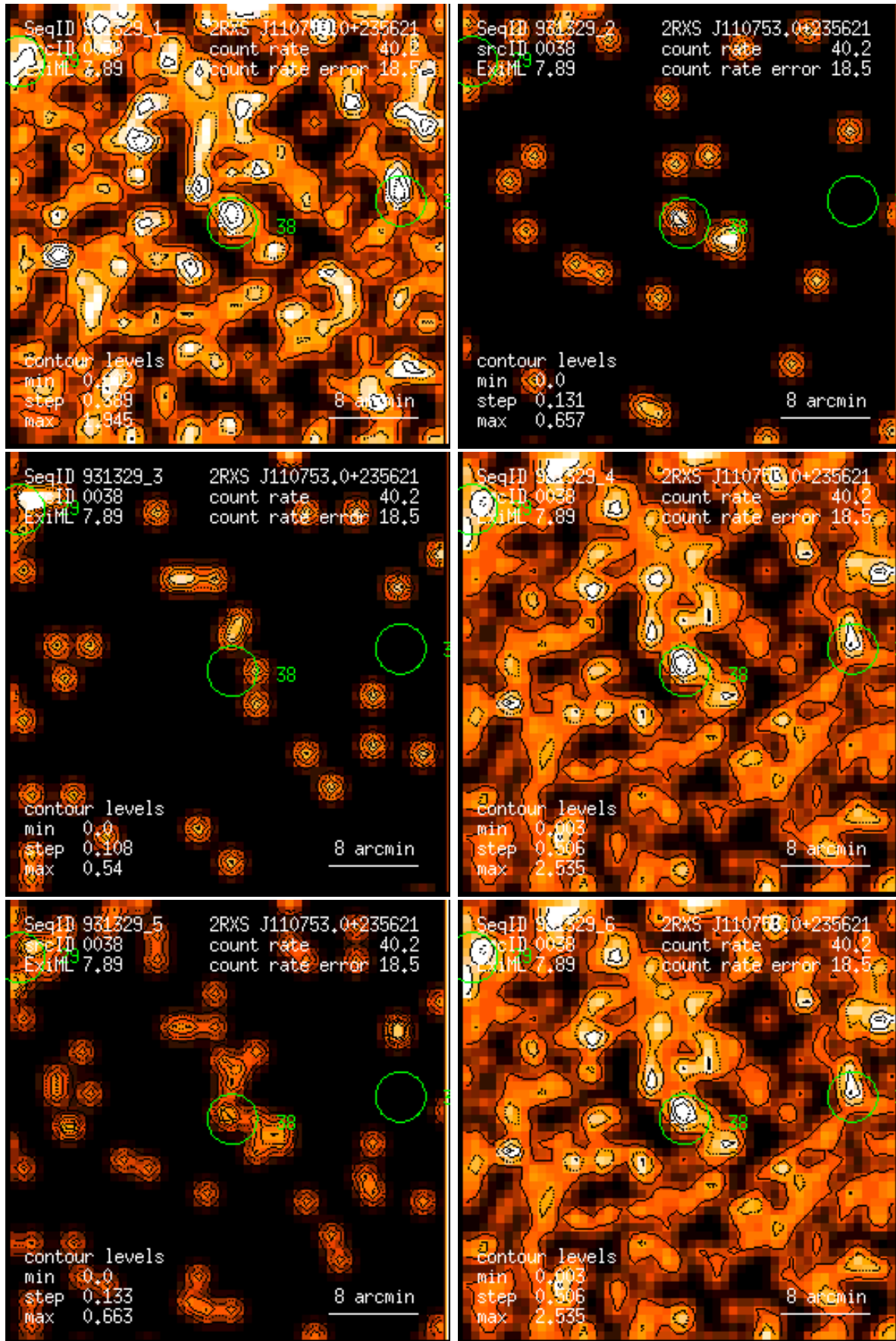
Figure 38: RASS 931329: detection 0038: band rate images, Gaussian filter: (1) PSPC channels 11 – 41, (2) 52 – 90, (3) 91 – 201, (4) 11 – 235, (5) 52 – 201, (6) 11 – 201. Broad band rates in counts/ks. Band rate contour levels in counts/ks/arcmin 2 .
