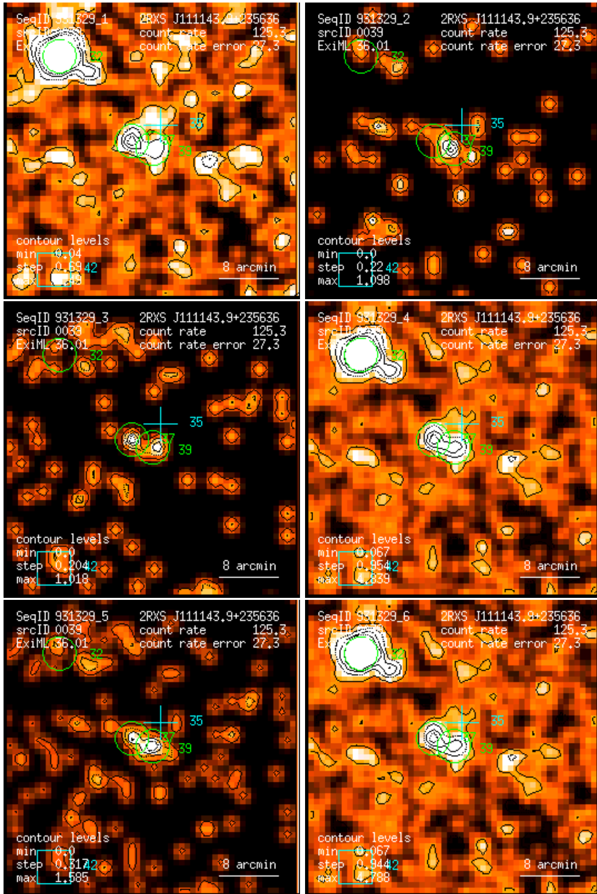
Figure 39: RASS 931329: detection 0039: band rate images, Gaussian filter: (1) PSPC channels 11 – 41, (2) 52 – 90, (3) 91 – 201, (4) 11 – 235, (5) 52 – 201, (6) 11 – 201. Broad band rates in counts/ks. Band rate contour levels in counts/ks/arcmin 2 .
