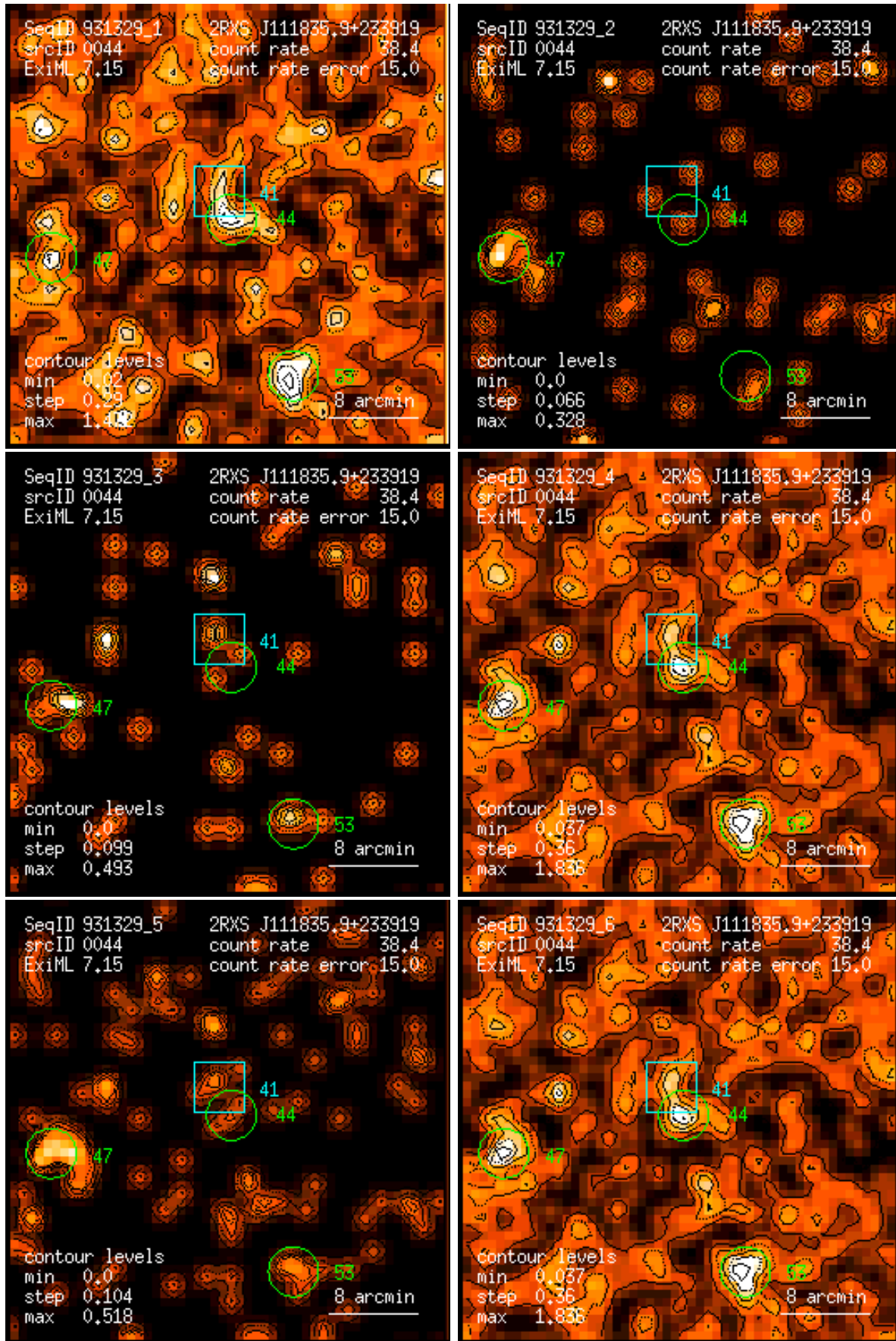
Figure 44: RASS 931329: detection 0044: band rate images, Gaussian filter: (1) PSPC channels 11 – 41, (2) 52 – 90, (3) 91 – 201, (4) 11 – 235, (5) 52 – 201, (6) 11 – 201. Broad band rates in counts/ks. Band rate contour levels in counts/ks/arcmin 2 .
