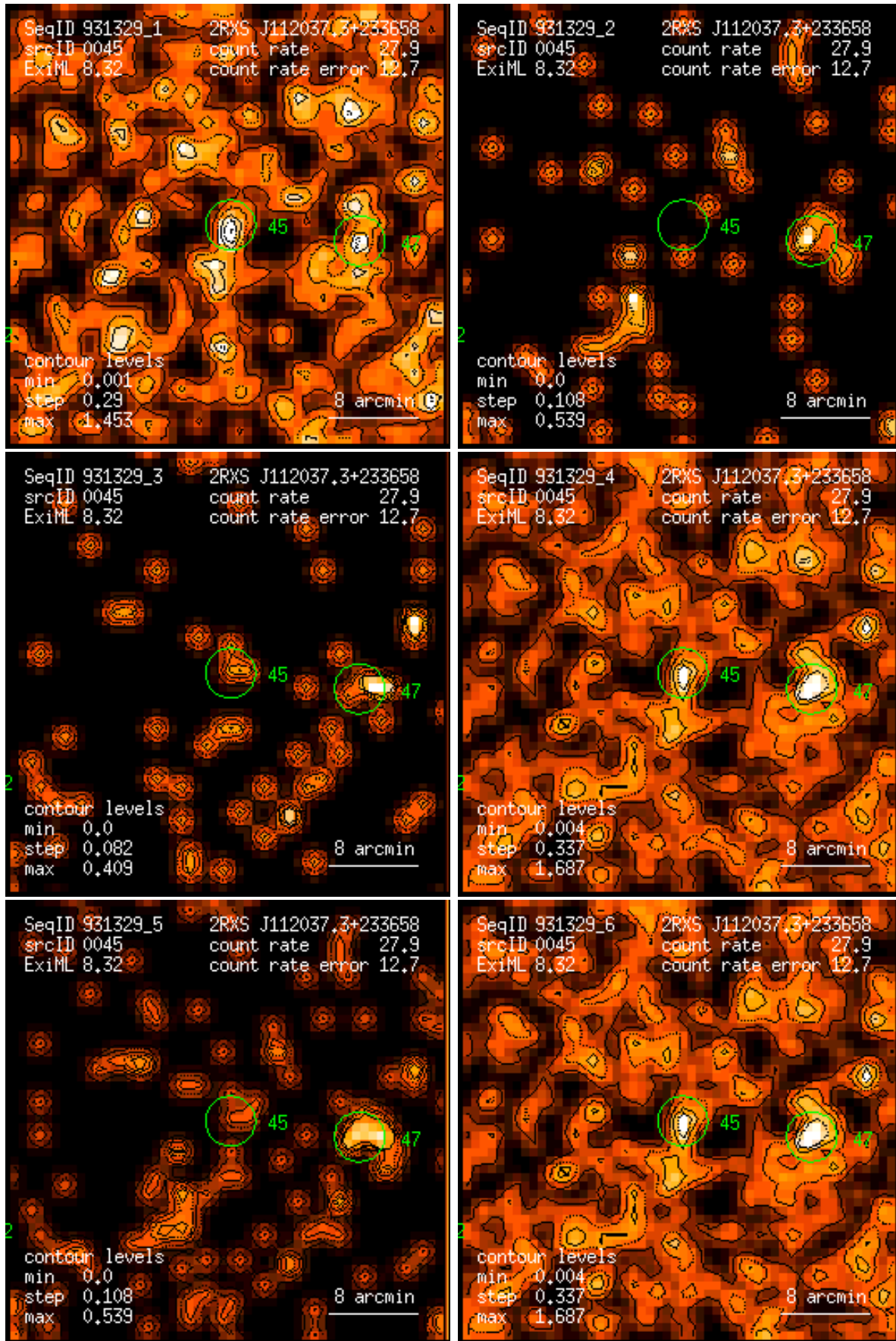
Figure 45: RASS 931329: detection 0045: band rate images, Gaussian filter: (1) PSPC channels 11 – 41, (2) 52 – 90, (3) 91 – 201, (4) 11 – 235, (5) 52 – 201, (6) 11 – 201. Broad band rates in counts/ks. Band rate contour levels in counts/ks/arcmin 2 .
