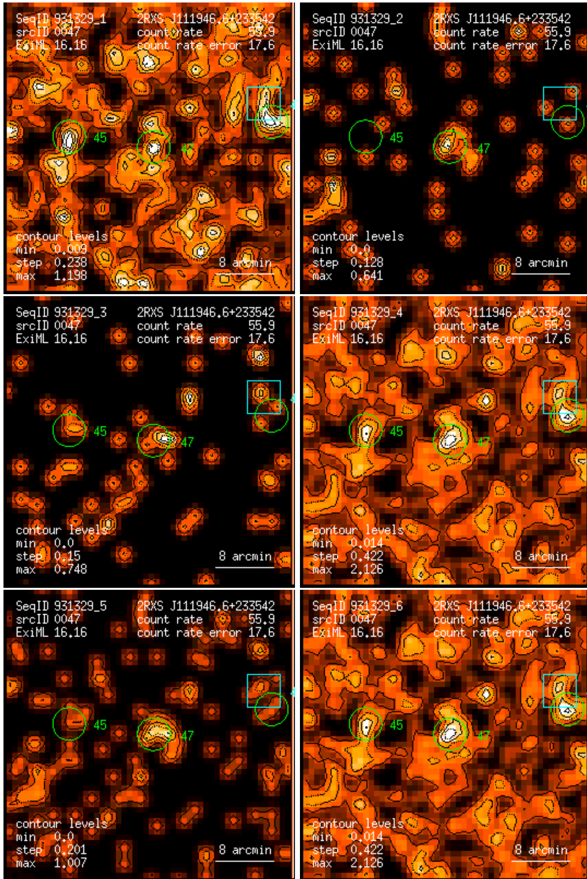
Figure 47: RASS 931329: detection 0047: band rate images, Gaussian filter: (1) PSPC channels 11 – 41, (2) 52 – 90, (3) 91 – 201, (4) 11 – 235, (5) 52 – 201, (6) 11 – 201. Broad band rates in counts/ks. Band rate contour levels in counts/ks/arcmin 2 .
