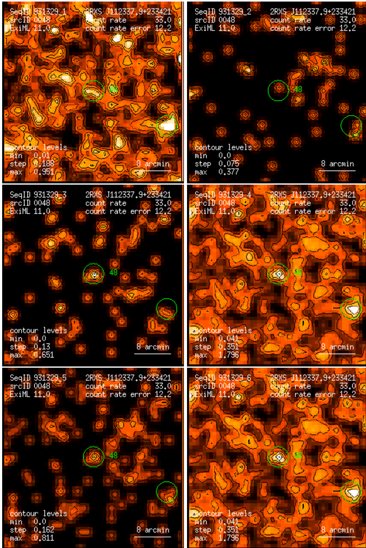
Figure 48: RASS 931329: detection 0048: band rate images, Gaussian filter: (1) PSPC channels 11 – 41, (2) 52 – 90, (3) 91 – 201, (4) 11 – 235, (5) 52 – 201, (6) 11 – 201. Broad band rates in counts/ks. Band rate contour levels in counts/ks/arcmin 2 .
