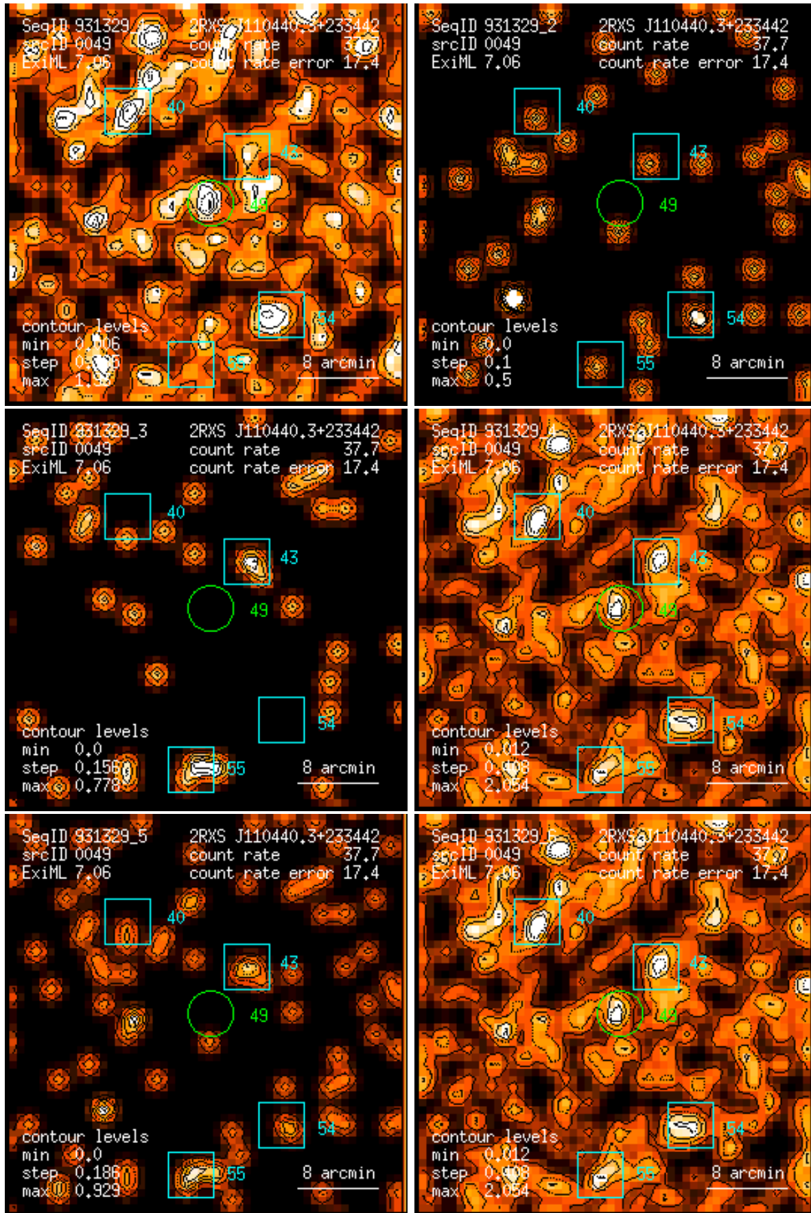
Figure 49: RASS 931329: detection 0049: band rate images, Gaussian filter: (1) PSPC channels 11 – 41, (2) 52 – 90, (3) 91 – 201, (4) 11 – 235, (5) 52 – 201, (6) 11 – 201. Broad band rates in counts/ks. Band rate contour levels in counts/ks/arcmin 2 .
