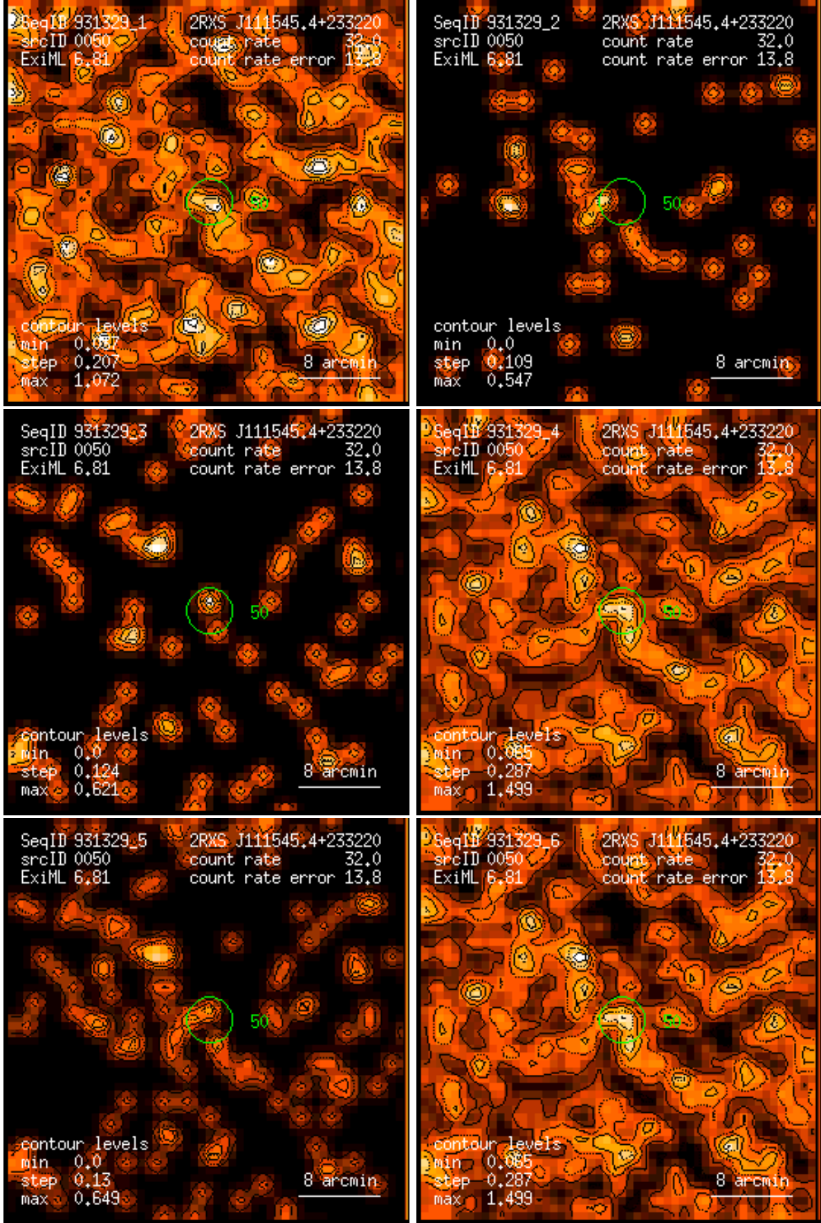
Figure 50: RASS 931329: detection 0050: band rate images, Gaussian filter: (1) PSPC channels 11 – 41, (2) 52 – 90, (3) 91 – 201, (4) 11 – 235, (5) 52 – 201, (6) 11 – 201. Broad band rates in counts/ks. Band rate contour levels in counts/ks/arcmin 2 .
