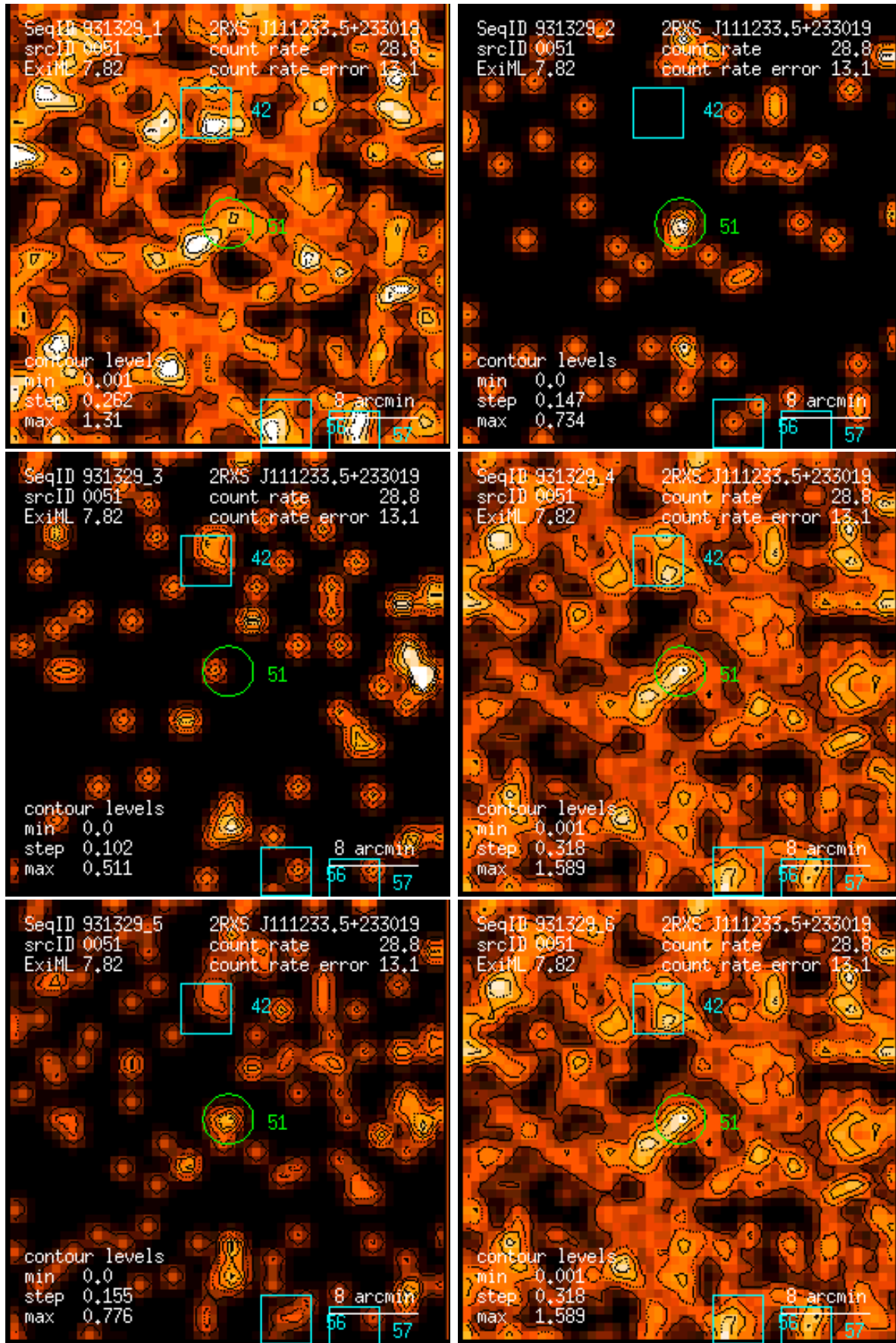
Figure 51: RASS 931329: detection 0051: band rate images, Gaussian filter: (1) PSPC channels 11 – 41, (2) 52 – 90, (3) 91 – 201, (4) 11 – 235, (5) 52 – 201, (6) 11 – 201. Broad band rates in counts/ks. Band rate contour levels in counts/ks/arcmin 2 .
