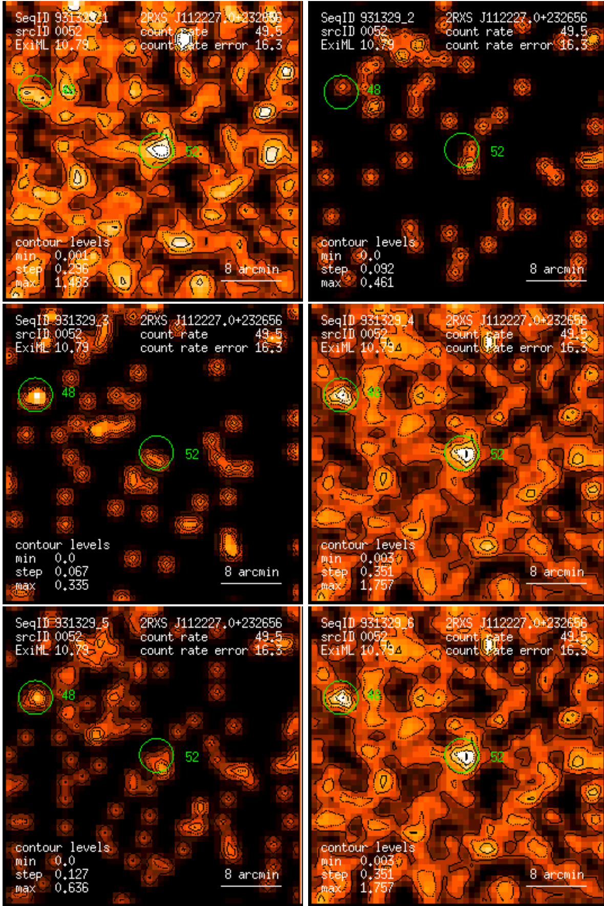
Figure 52: RASS 931329: detection 0052: band rate images, Gaussian filter: (1) PSPC channels 11 – 41, (2) 52 – 90, (3) 91 – 201, (4) 11 – 235, (5) 52 – 201, (6) 11 – 201. Broad band rates in counts/ks. Band rate contour levels in counts/ks/arcmin 2 .
