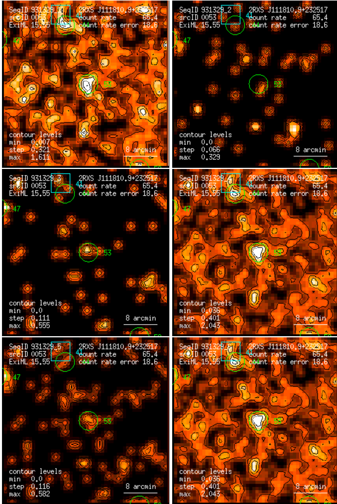
Figure 53: RASS 931329: detection 0053: band rate images, Gaussian filter: (1) PSPC channels 11 – 41, (2) 52 – 90, (3) 91 – 201, (4) 11 – 235, (5) 52 – 201, (6) 11 – 201. Broad band rates in counts/ks. Band rate contour levels in counts/ks/arcmin 2 .
