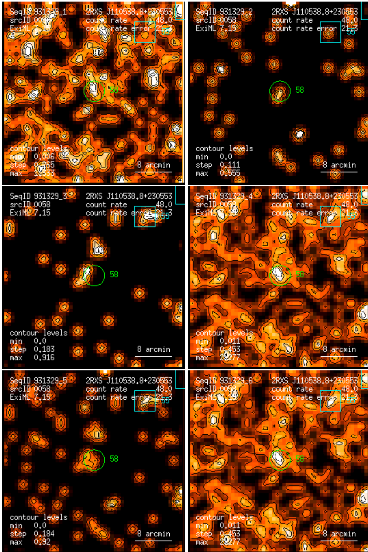
Figure 58: RASS 931329: detection 0058: band rate images, Gaussian filter: (1) PSPC channels 11 – 41, (2) 52 – 90, (3) 91 – 201, (4) 11 – 235, (5) 52 – 201, (6) 11 – 201. Broad band rates in counts/ks. Band rate contour levels in counts/ks/arcmin 2 .
