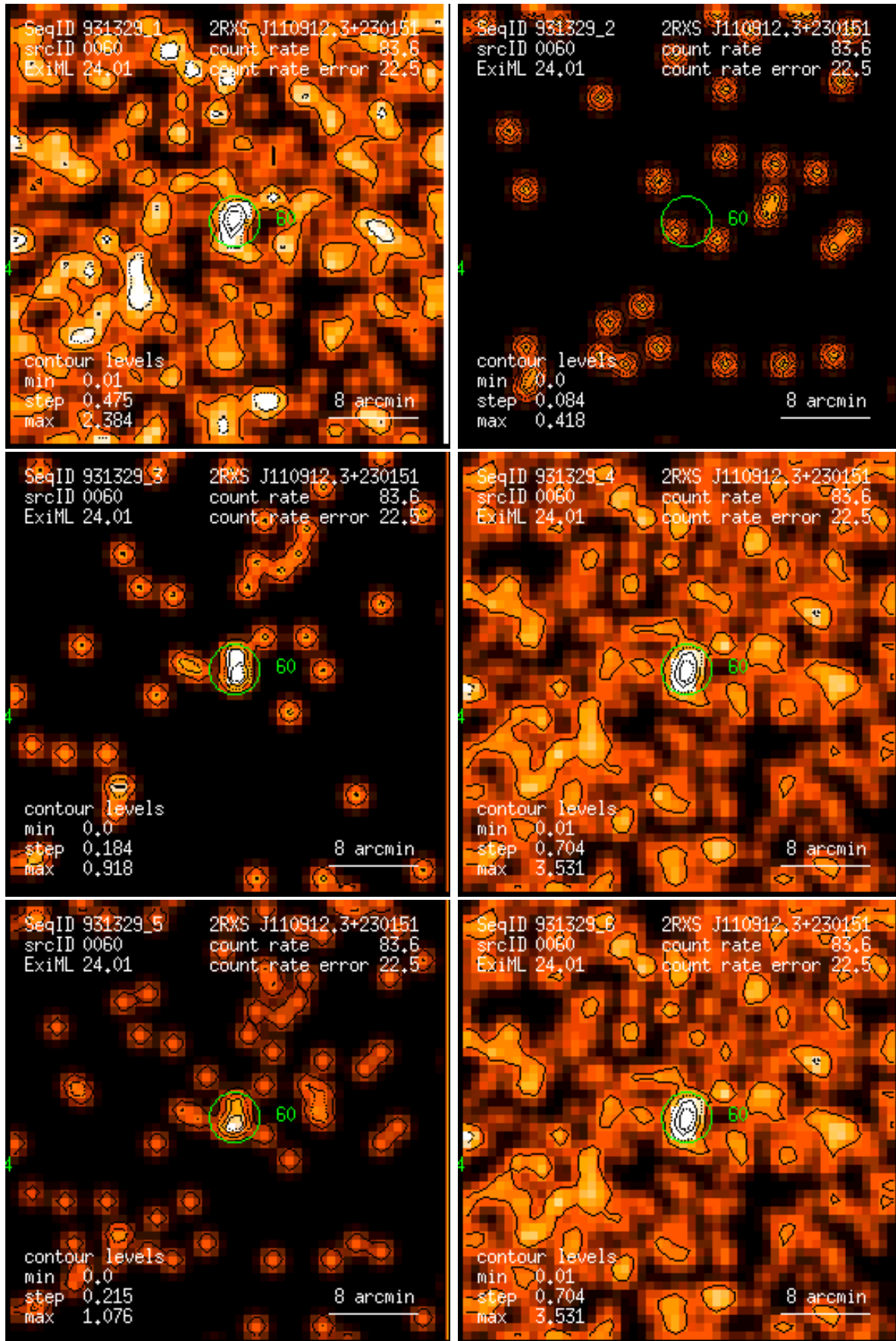
Figure 60: RASS 931329: detection 0060: band rate images, Gaussian filter: (1) PSPC channels 11 – 41, (2) 52 – 90, (3) 91 – 201, (4) 11 – 235, (5) 52 – 201, (6) 11 – 201. Broad band rates in counts/ks. Band rate contour levels in counts/ks/arcmin 2 .
