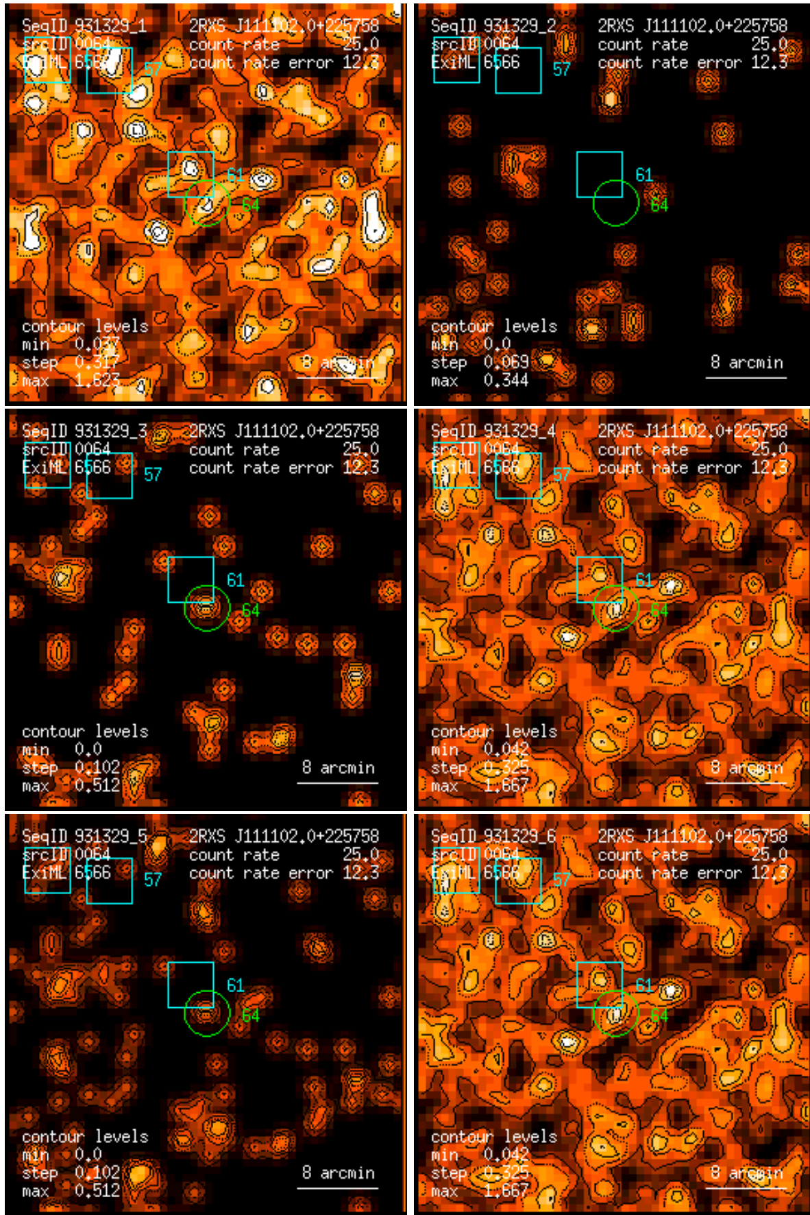
Figure 64: RASS 931329: detection 0064: band rate images, Gaussian filter: (1) PSPC channels 11 – 41, (2) 52 – 90, (3) 91 – 201, (4) 11 – 235, (5) 52 – 201, (6) 11 – 201. Broad band rates in counts/ks. Band rate contour levels in counts/ks/arcmin 2 .
