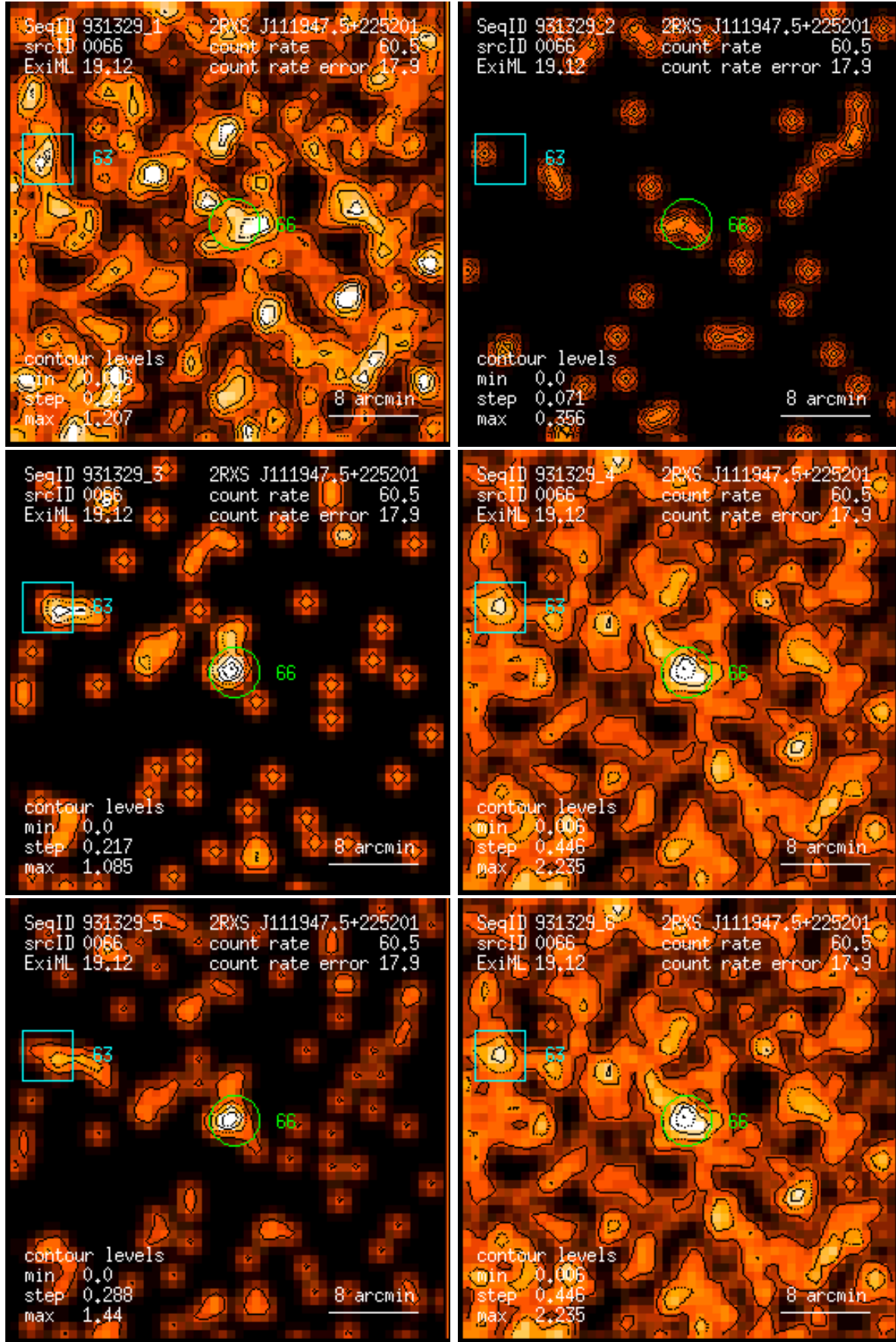
Figure 66: RASS 931329: detection 0066: band rate images, Gaussian filter: (1) PSPC channels 11 – 41, (2) 52 – 90, (3) 91 – 201, (4) 11 – 235, (5) 52 – 201, (6) 11 – 201. Broad band rates in counts/ks. Band rate contour levels in counts/ks/arcmin 2 .
