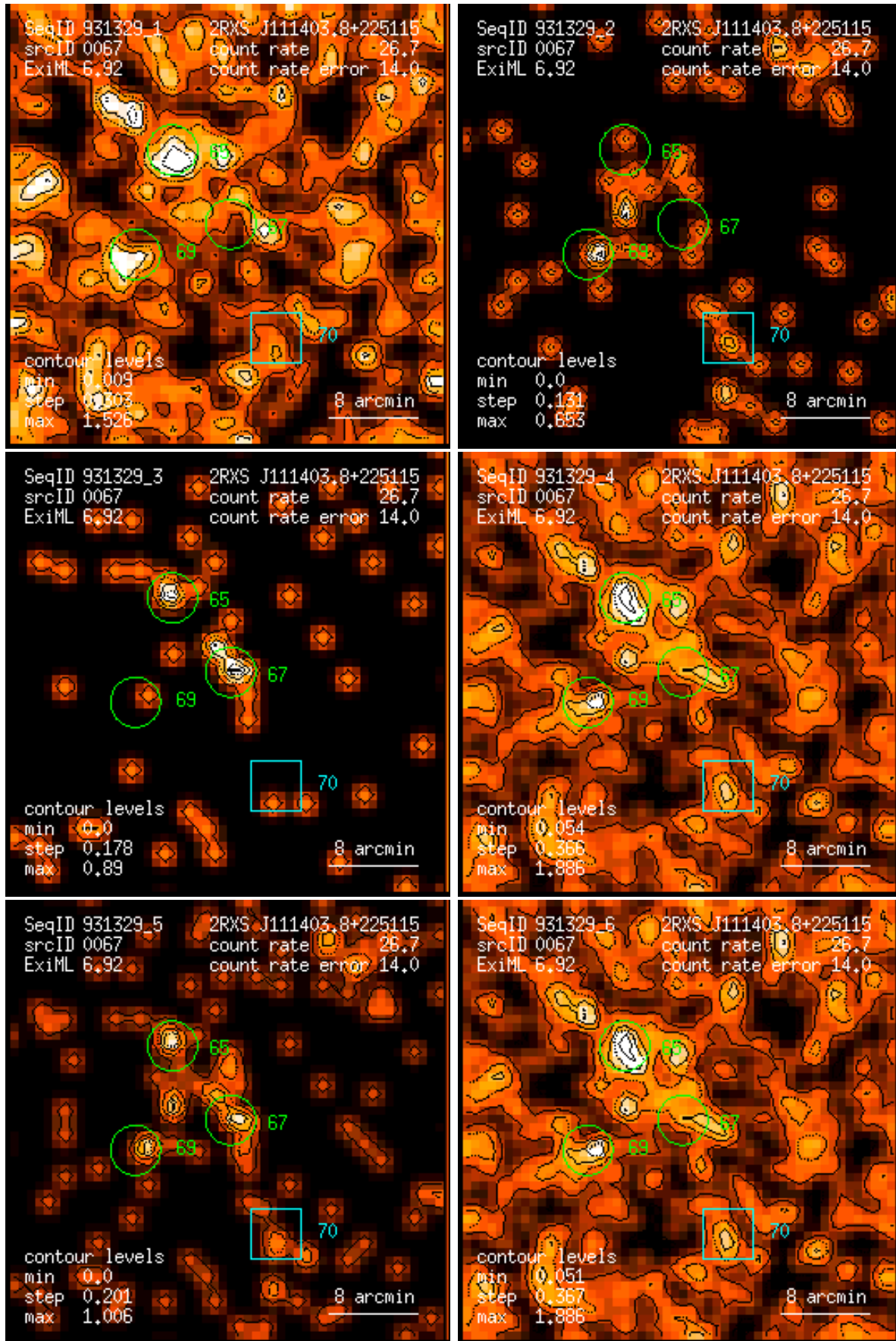
Figure 67: RASS 931329: detection 0067: band rate images, Gaussian filter: (1) PSPC channels 11 – 41, (2) 52 – 90, (3) 91 – 201, (4) 11 – 235, (5) 52 – 201, (6) 11 – 201. Broad band rates in counts/ks. Band rate contour levels in counts/ks/arcmin 2 .
