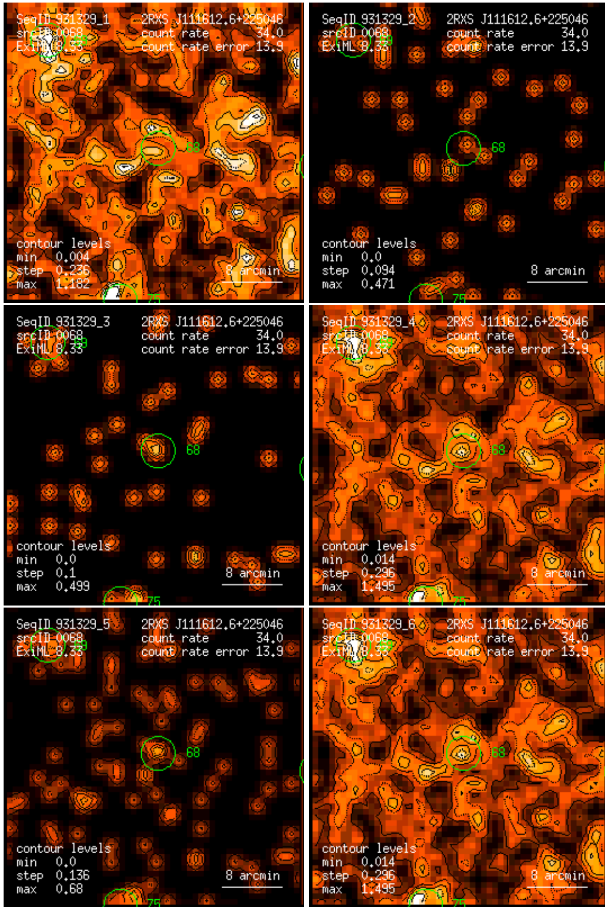
Figure 68: RASS 931329: detection 0068: band rate images, Gaussian filter: (1) PSPC channels 11 – 41, (2) 52 – 90, (3) 91 – 201, (4) 11 – 235, (5) 52 – 201, (6) 11 – 201. Broad band rates in counts/ks. Band rate contour levels in counts/ks/arcmin 2 .
