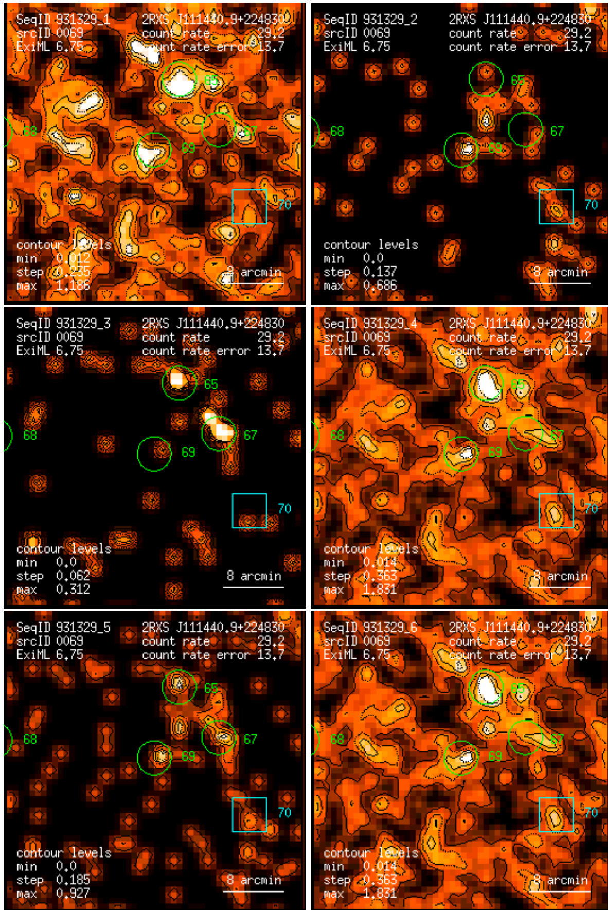
Figure 69: RASS 931329: detection 0069: band rate images, Gaussian filter: (1) PSPC channels 11 – 41, (2) 52 – 90, (3) 91 – 201, (4) 11 – 235, (5) 52 – 201, (6) 11 – 201. Broad band rates in counts/ks. Band rate contour levels in counts/ks/arcmin 2 .
