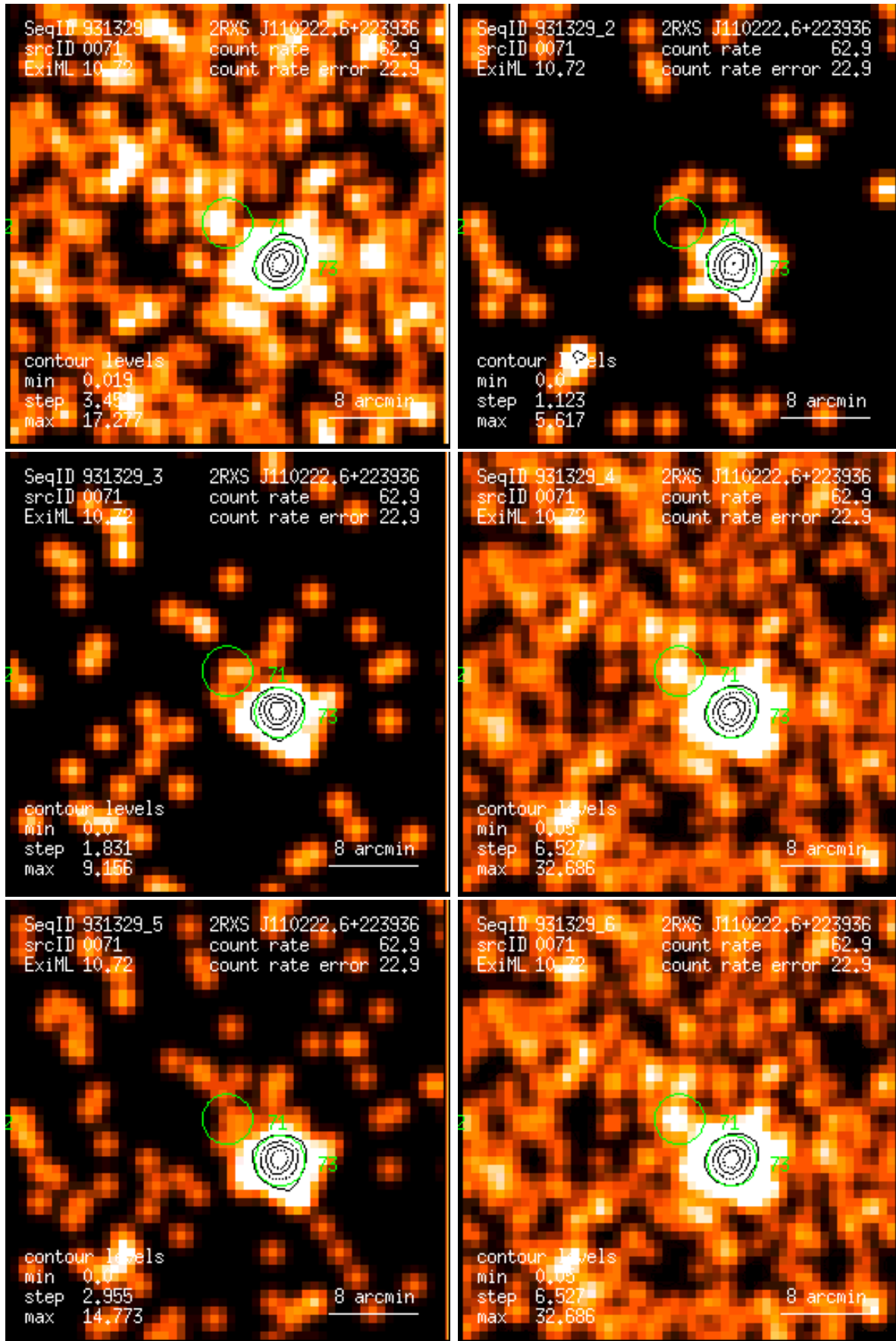
Figure 71: RASS 931329: detection 0071: band rate images, Gaussian filter: (1) PSPC channels 11 – 41, (2) 52 – 90, (3) 91 – 201, (4) 11 – 235, (5) 52 – 201, (6) 11 – 201. Broad band rates in counts/ks. Band rate contour levels in counts/ks/arcmin 2 .
